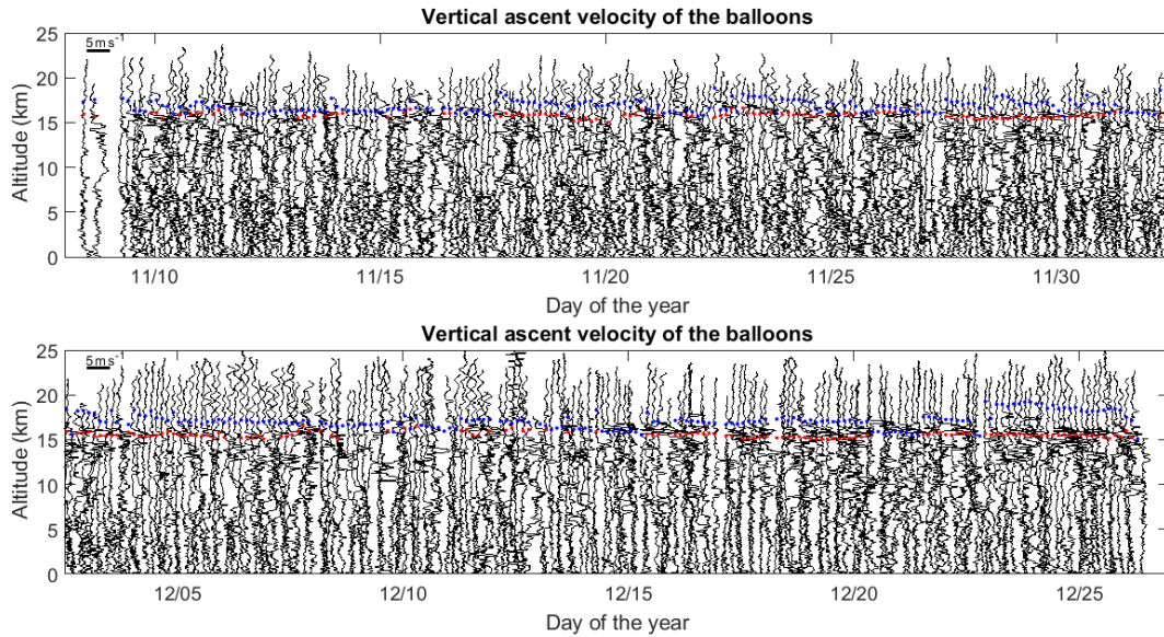
Figure 8. Vertical profiles of V_B from 376 consecutive balloons launched about every 3 h from 8 November to 27 December 2015 during the pre-YMC campaign at Bengkulu ( 102.26^\circ E, 3.79^\circ S; Indonesia); 0.5 d corresponds to 5 \text{ m s}^{-1} , and each profile was shifted by about 0.125 d ( 1.25 \text{ m s}^{-1} ). The cold point temperature tropopause and a secondary temperature inversion of similar intensity at lower altitude are shown as blue and red dots, respectively.
