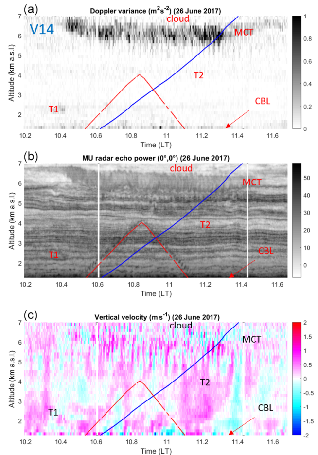
Figure 2. (a) Time–height cross section of variance of the Doppler spectrum peaks corrected from the beam-broadening effects obtained from MU radar measurements during balloon flight V14 and UAV flight SH29. The altitudes of V14 and SH29 vs. time are given by blue and red lines, respectively. (b) Same as top for radar echo power (dB) in range imaging mode. (c) Same as top for vertical velocity ( \text{m s}^{-1} ). The white vertical lines are due to radar stops. See, e.g., Luce et al. (2018) for more details about these figures. Labels refer to the location of turbulent layers.
