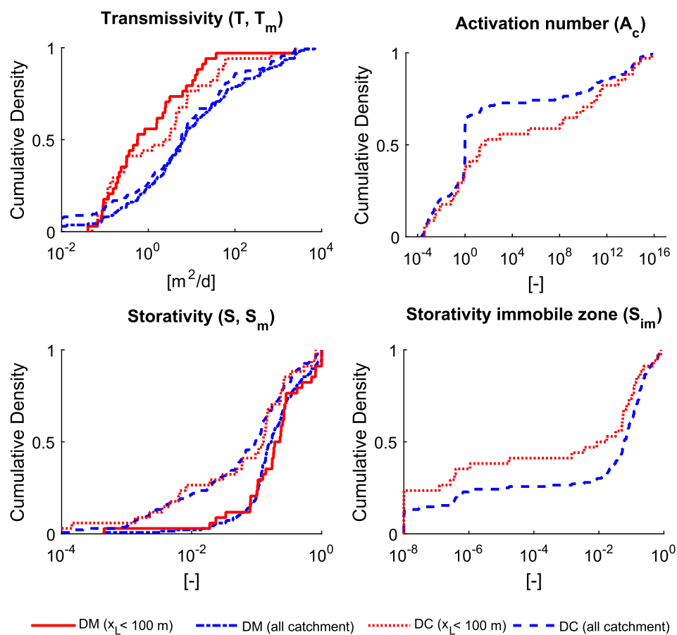
Figure 5. Cumulative distributions of (top left) transmissivities, (top right) activation number A_c , (bottom) storativity. Estimates from the DM are (red solid) for x_L < 100 m and (blue dash-dotted) for the all the catchment. Estimates from the nonlocal DM (DC) are (red dotted) for x_L < 100 m and (blue dashed) for the whole catchment.
