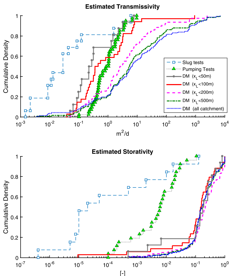
Figure 3. (top) Cumulative distributions of transmissivity ( T , in \text{m}^2/\text{d} ) and (bottom) storativity ( S , dimensionless) obtained from (squares) slug tests, (triangles) pumping tests, and from fitting of experimental TFs with the DM associated to boreholes located at (gray circles) x_L < 0.05 , (red solid) x_L < 0.1 , (pink dashed) x_L < 0.2 , (green dash-dotted) x_L < 0.5 , and (blue dotted) data from the whole catchment.
