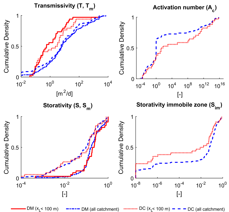
Figure 5. Cumulative distributions of (top left) transmissivities, (top right) activation number A_c , (bottom) storativity. Estimates from the DM are (red solid) for x_L < 100 m and (blue dash-dotted) for the all the catchment. Estimates from the nonlocal DM (DC) are (red dotted) for x_L < 100 m and (blue dashed) for the whole catchment.
