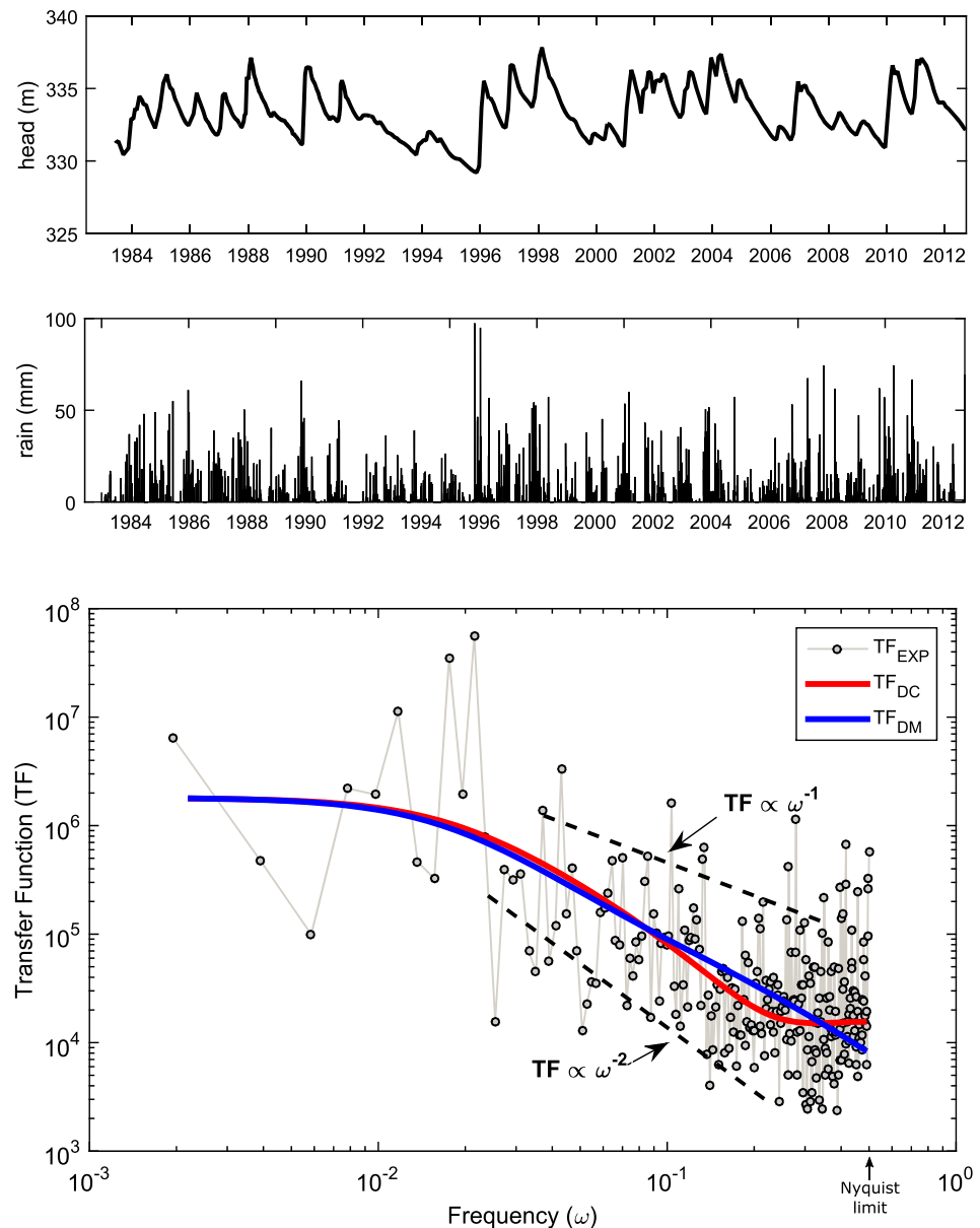
Figure 4. From top to bottom, a representative example of the hydrograph from one selected borehole, the rainfall time series and the resulting experimental transfer function ( TF_{EXP} ), with the fitted models (DM = single-porosity, scale-dependent DM; DC = dual-continuum version of the DM).
