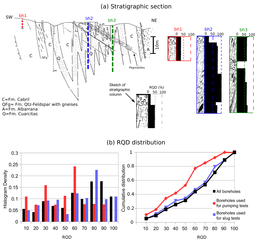
Figure 2. (a) Geological sketch of El Cabril (oriented NE-SW) and three representative stratigraphic columns with vertical distribution of the corresponding logs and the calculated RQD values; (b) frequency histogram and cumulative density of RQD at the El Cabril site. Black colors refer to the distribution obtained from all existing data; red and blue refer to distributions obtained from the subsample of boreholes used for pumping and slug tests, respectively.
