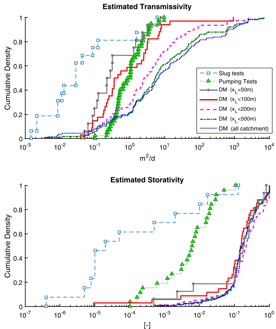
Figure 3. (top) Cumulative distributions of transmissivity ( T , in m^2/d ) and (bottom) storativity ( S , dimensionless) obtained from (squares) slug tests, (triangles) pumping tests, and from fitting of experimental TFs with the DM associated to boreholes located at (gray circles) x_L < 0.05 , (red solid) x_L < 0.1 , (pink dashed) x_L < 0.2 , (green dash-dotted) x_L < 0.5 , and (blue dotted) data from the whole catchment.
