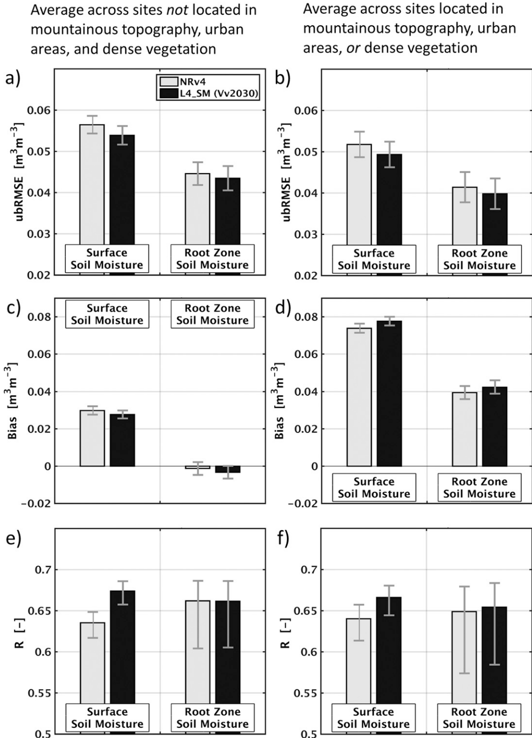
FIG. 9. (a),(b) ubRMSE ( m^3 m^{-3} ); (c),(d) bias ( m^3 m^{-3} ); and (e),(f) R (dimensionless) for L4_SM and NRv4 surface and root-zone soil moisture vs sparse network measurements, averaged across sites (left) within the mask and (right) outside the mask shown by the gray shading in Figs. 7 and 8. Averages are based on a clustering algorithm (section 3c). Error bars indicate 95% confidence intervals.
