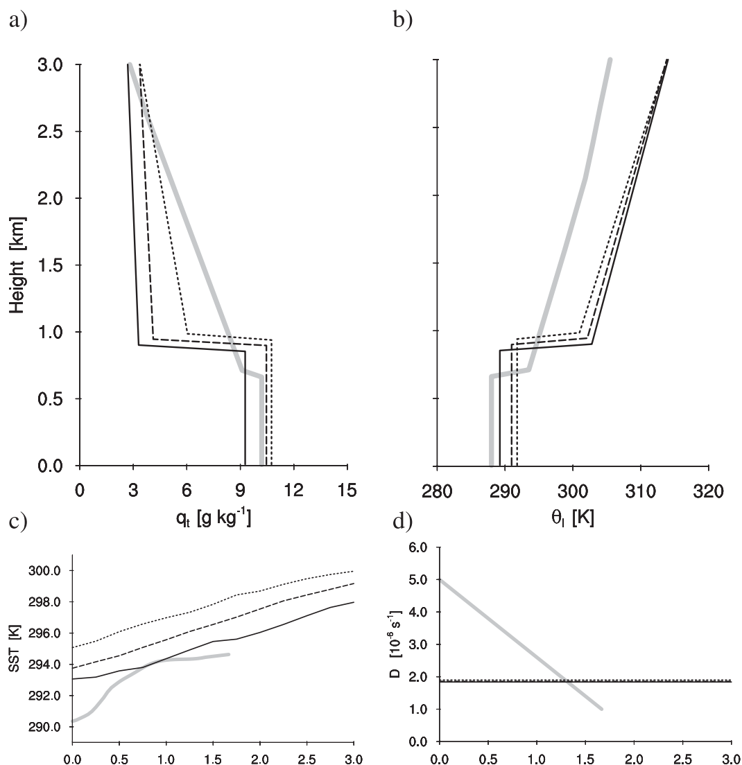
Figure 2. Defining aspects of the setup of the four transition cases. Figures 2a and 2b show the initial profiles of total specific humidity q_t , and the liquid water potential temperature \theta_l , while Figures 2c and 2d show the time series of the prescribed SST and the large-scale divergence. The solid grey line represents the ASTEX case, while the SLOW, REF, and FAST composite cases are plotted as solid, dashed, and dotted black lines, respectively.
