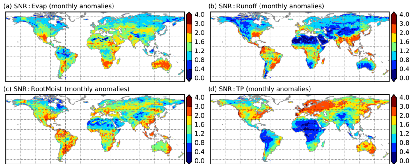
Figure 2. Signal-to-noise ratio of monthly mean anomalies of evapotranspiration (a), runoff (b), root zone soil moisture (c) and precipitation (d).
