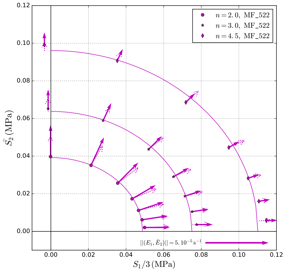
Figure 5. Influence of the exponent n onto the iso-dissipation curves ( \mathcal{P}_v = \mathcal{P}_v^o ) for the particular snow sample MF_{522} . The associated strain flow vectors ( \bar{E}_1^o, \bar{E}_2^o ) are represented by solid arrows. Abouaf models are fitted to the numerical points (solid lines) and theoretical values of strain flow vectors are shown (dashed arrows).
