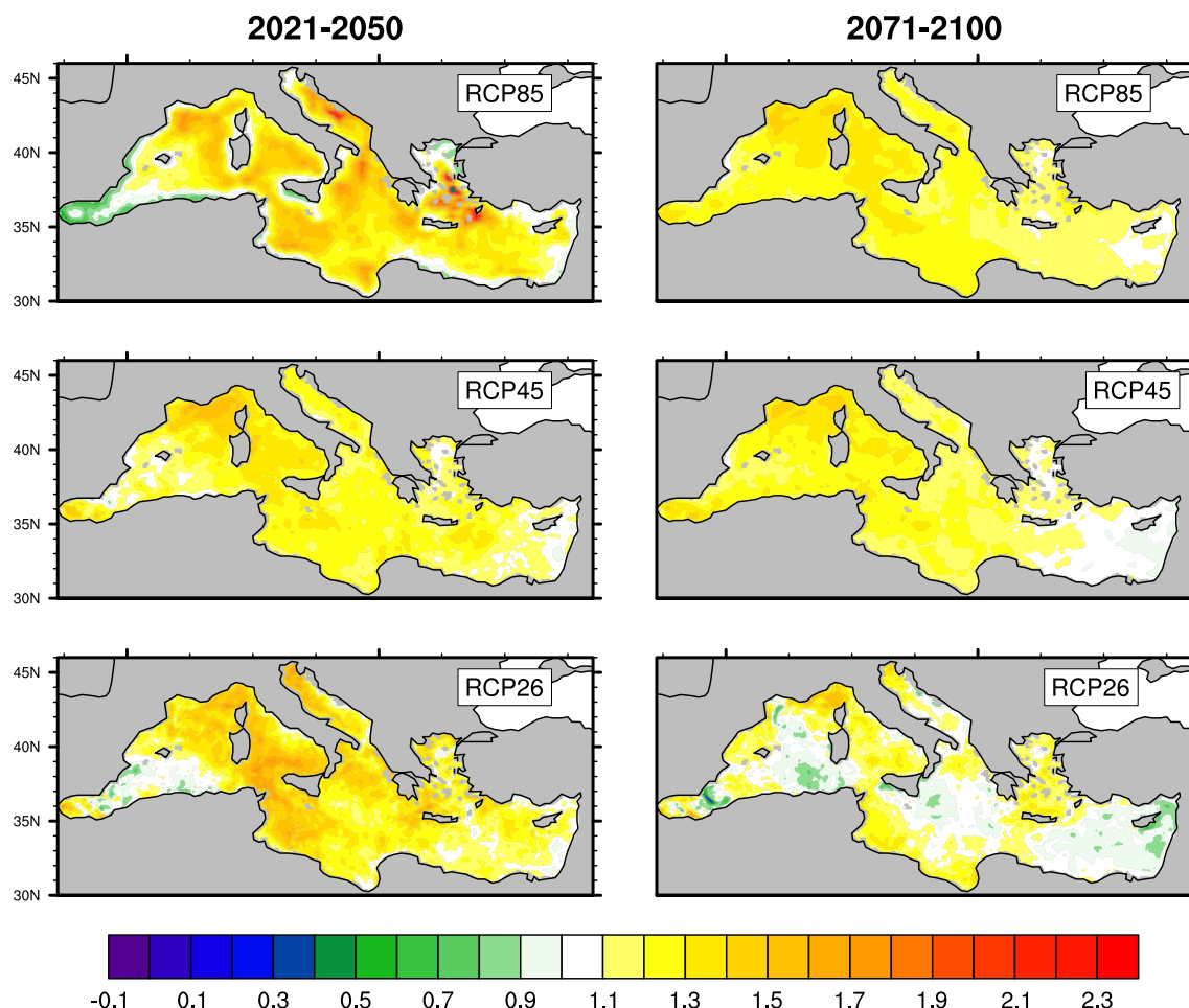
Fig. 13 Multi-model mean ratio R of \Delta SST_{99Q} (°C) over \Delta \overline{SST} (°C) for every period and scenario. Regions where R > 1/R < 1 indicate
