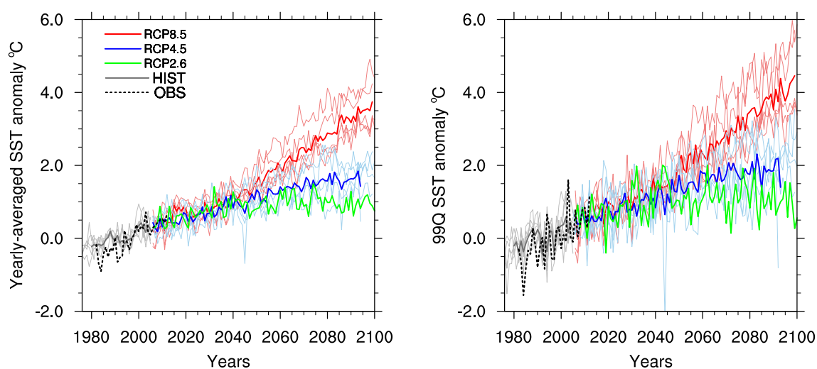
Fig. 6 Area-average, yearly \overline{SST} °C (left) and extreme \overline{SST}_{99Q} °C (right) anomalies with respect to HIST. Bold colors represent the
