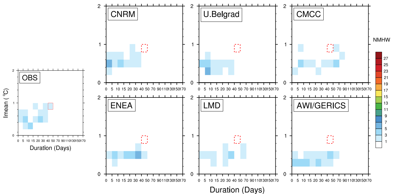
Fig. 5 IDF plot; Intensity ( I_{\text{mean}} in °C), Duration (Days), Frequency (Number of MHW during 1976–2005). I_{\text{mean}} is organised in bins of 0.02 °C while duration is in bins of 5, 10 and 20 days. Red box indicates observed characteristics corresponding to the exceptional MHW of 2003
