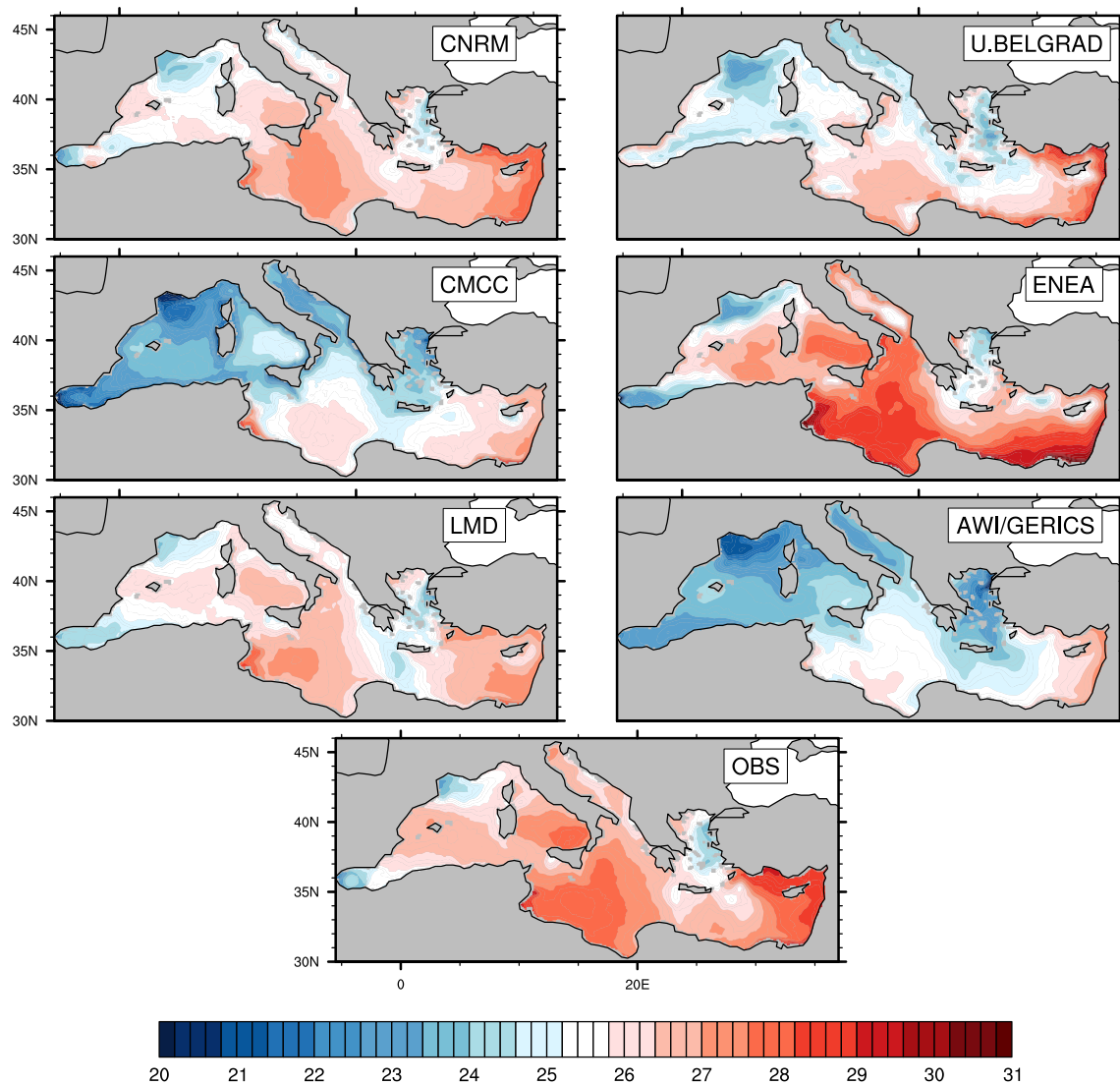
Fig. 3 Individual MHW threshold maps of mean SST 99Q (°C) computed from the HIST run of every model (1976–2005) and satellite data during 1982–2012. Note that the HIST run for ENEA is from 1979–2005
