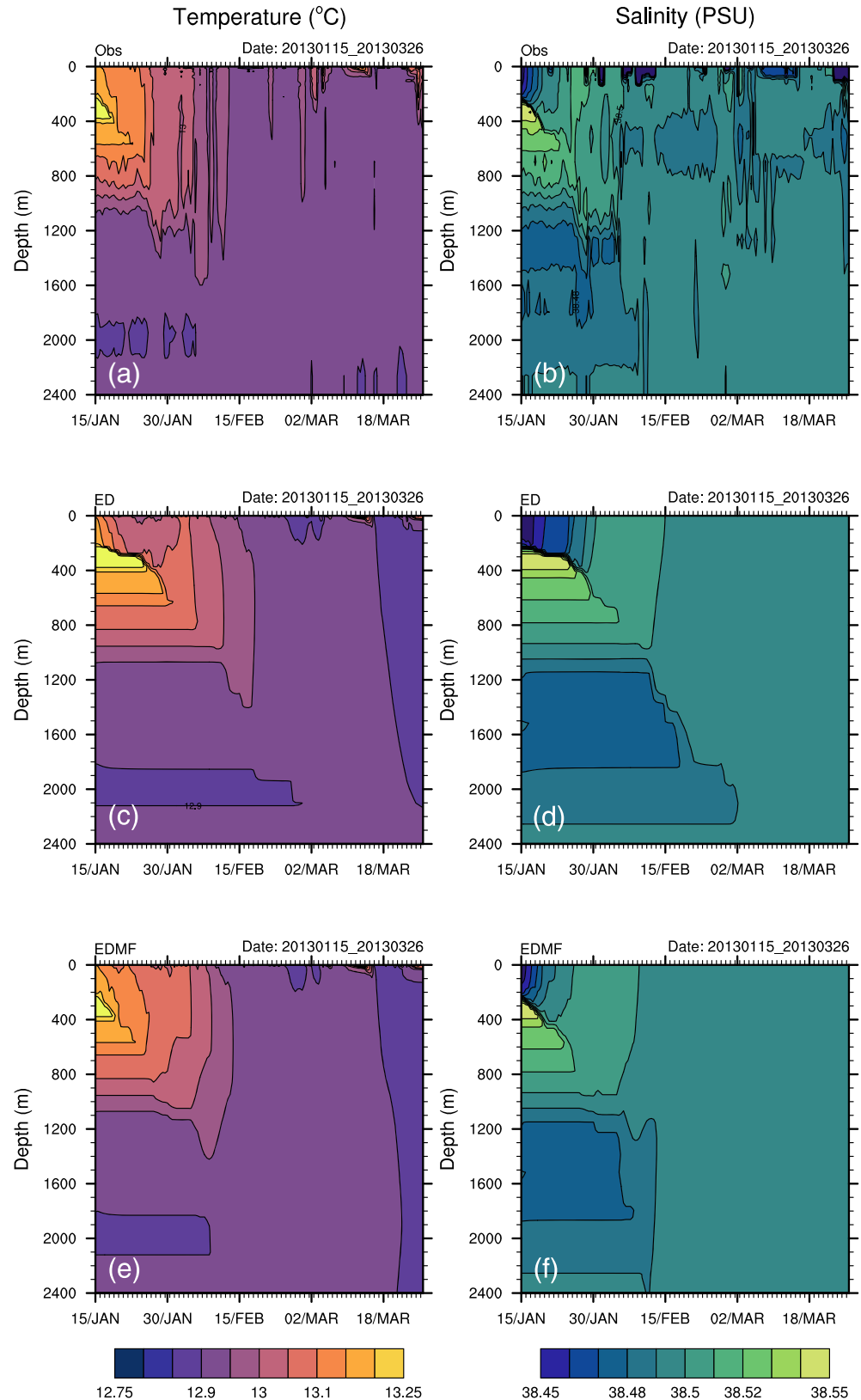
Figure 6. Time series at the Lion buoy of temperature ( ^{\circ}\text{C} , left) and salinity ( \text{psu} , right) for (a,b) observation, (c,d) ED scheme, and (e,f) EDMF scheme.
