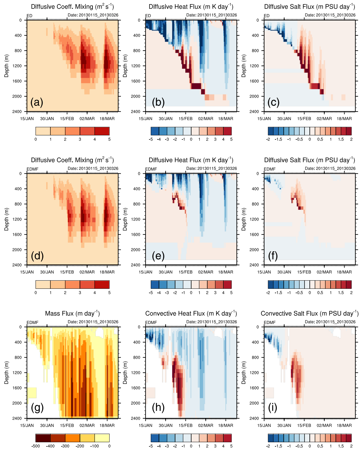
Figure 8. Time series at the Lion buoy of (a,d) the vertical coefficient mixing ( \text{m}^2 \text{s}^{-1} ), (g) the mass-flux ( \text{m day}^{-1} ), (b,e,h) the vertical heat flux ( \text{m K day}^{-1} ) and (c,f,i) the vertical haline flux ( \text{m psu day}^{-1} ) for the ED alone (top), ED in EDMF (middle) and Mass-Flux in EDMF (bottom) schemes.
