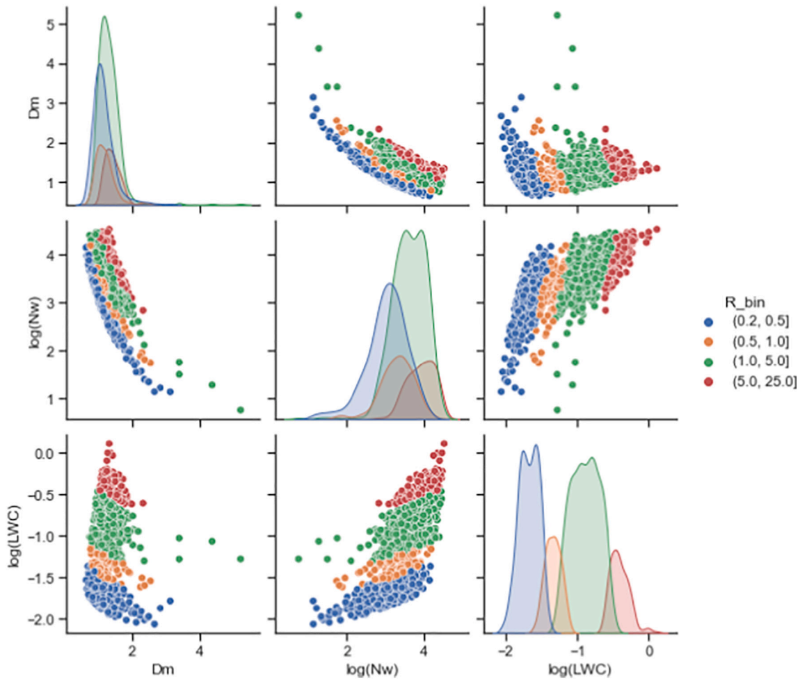
Fig. 5. Kernel Density Estimate (plots in the diagonal) and correlation (remaining plots) between D_m (mm), \log(N_w) (dimensionless) and \text{LWC} ( \text{g m}^{-3} ) for stripped rain rate ( \text{mm h}^{-1} ) of rainfall measured by Parsivel during the C2017.
