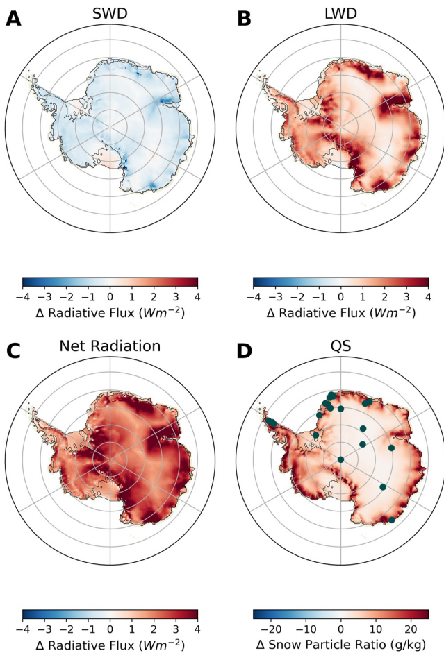
Figure 4. Difference in radiative components at the surface and snow particle ratio between MAR with and without drifting snow. (a) Difference in incoming shortwave radiation (SWD) at the surface in Wm^{-2} . Red color indicates a greater downwelling shortwave flux in MAR with active drifting snow parameterization. (b) Same (a) but for the downwelling longwave flux at the surface. (c) Same as (a) and (b), but for the difference in the net radiation at the surface ( R = SWD * (1 - \alpha) + LWD - LWU ). (d) Same as above but for the difference in snow particle content (g/kg), a measure of airborne drifting snow particles. Dots show the locations of the weather stations in our statistical comparison in Figure 5.
