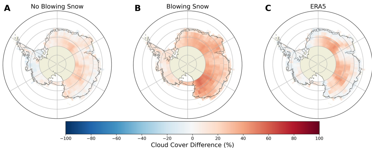
Figure 3. Comparison between Cloudsat-Calipso cloud cover, MAR and ERA5. (a) Comparison between MAR without drifting snow and Cloudsat-calipso cloud cover over 07/2006–02/2011. (b) Same as (a) but for the comparison with MAR including drifting snow. (c) Comparison between ERA5 cloud cover and the Cloudsat-Calipso cloud cover.
