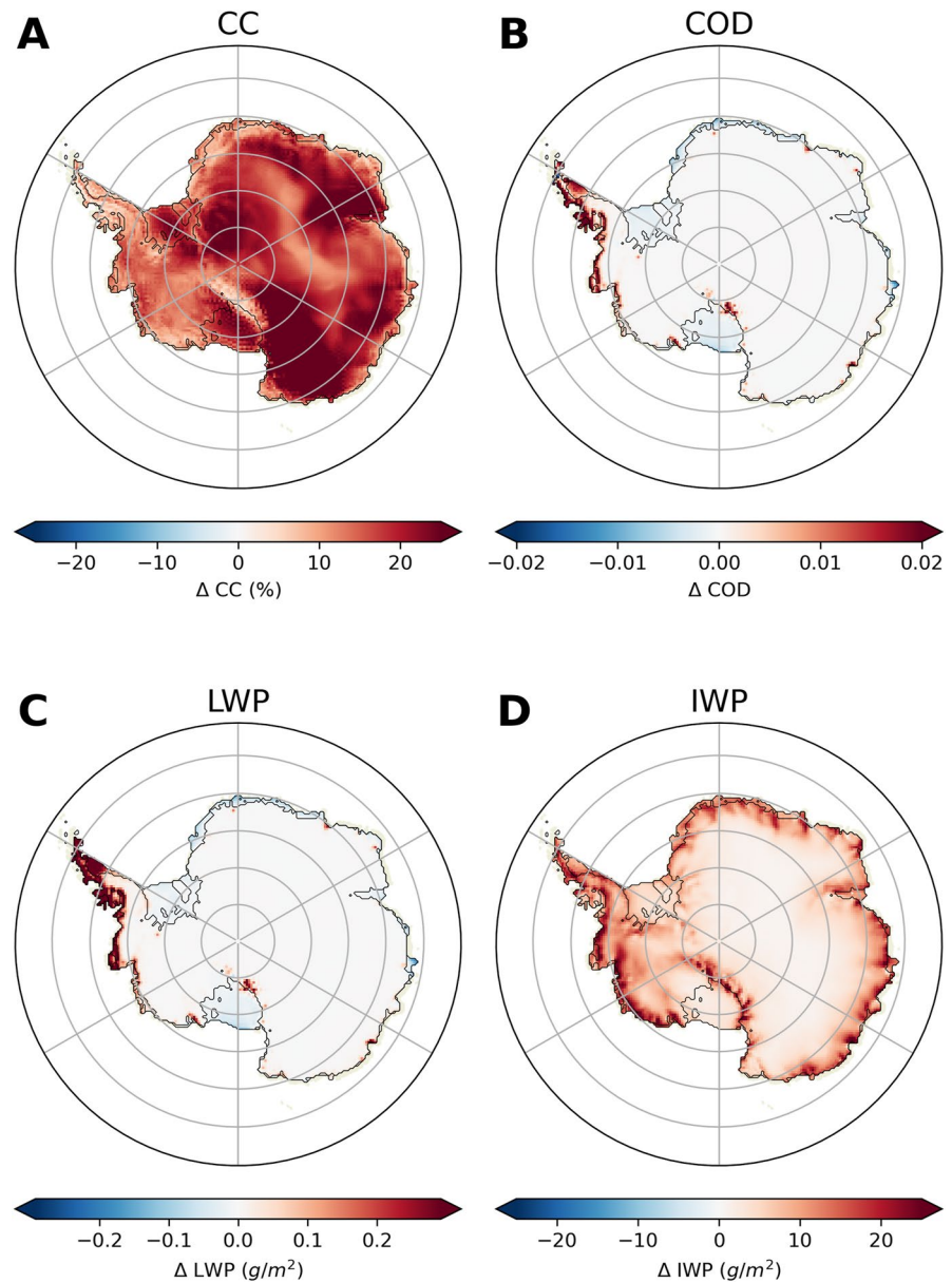
Figure 2. Difference in cloud properties between MAR with and without drifting snow. (a) Difference in cloud cover (%) between the two MAR simulations. Red colors indicate a greater cloud cover percentage in MAR with active drifting snow parameterization. (b) Same as (a) but for the difference in cloud optical depth (COD, unitless) between the two MAR simulations. (c) Same as (a) but for the difference in liquid water path (LWP, \text{g}/\text{m}^2 ). (d) Same as (a) but for the difference in ice water path (ice water path, \text{g}/\text{m}^2 ).
