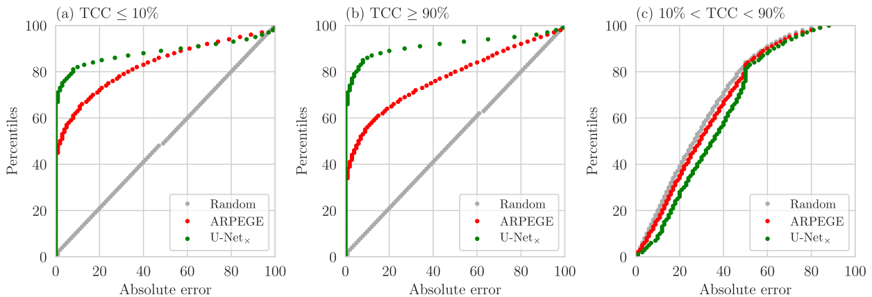
FIG. 11. Comparison of the cumulative distribution of absolute errors (%) in ARPEGE and the U-Net x relatively to the TCC value: (a) TCC \leq 10\% , (b) TCC \geq 90\% , and (c) 10\% < TCC < 90\% . The errors calculated on a randomly generated dataset are in gray.
