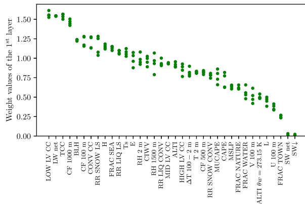
FIG. 13. Values of weight of the first layer added before the U-Net x . For each variable, the four values correspond to the four models trained for the cross validation. The variables are sorted by descending mean value. A description of the variables is given in Table 1.
