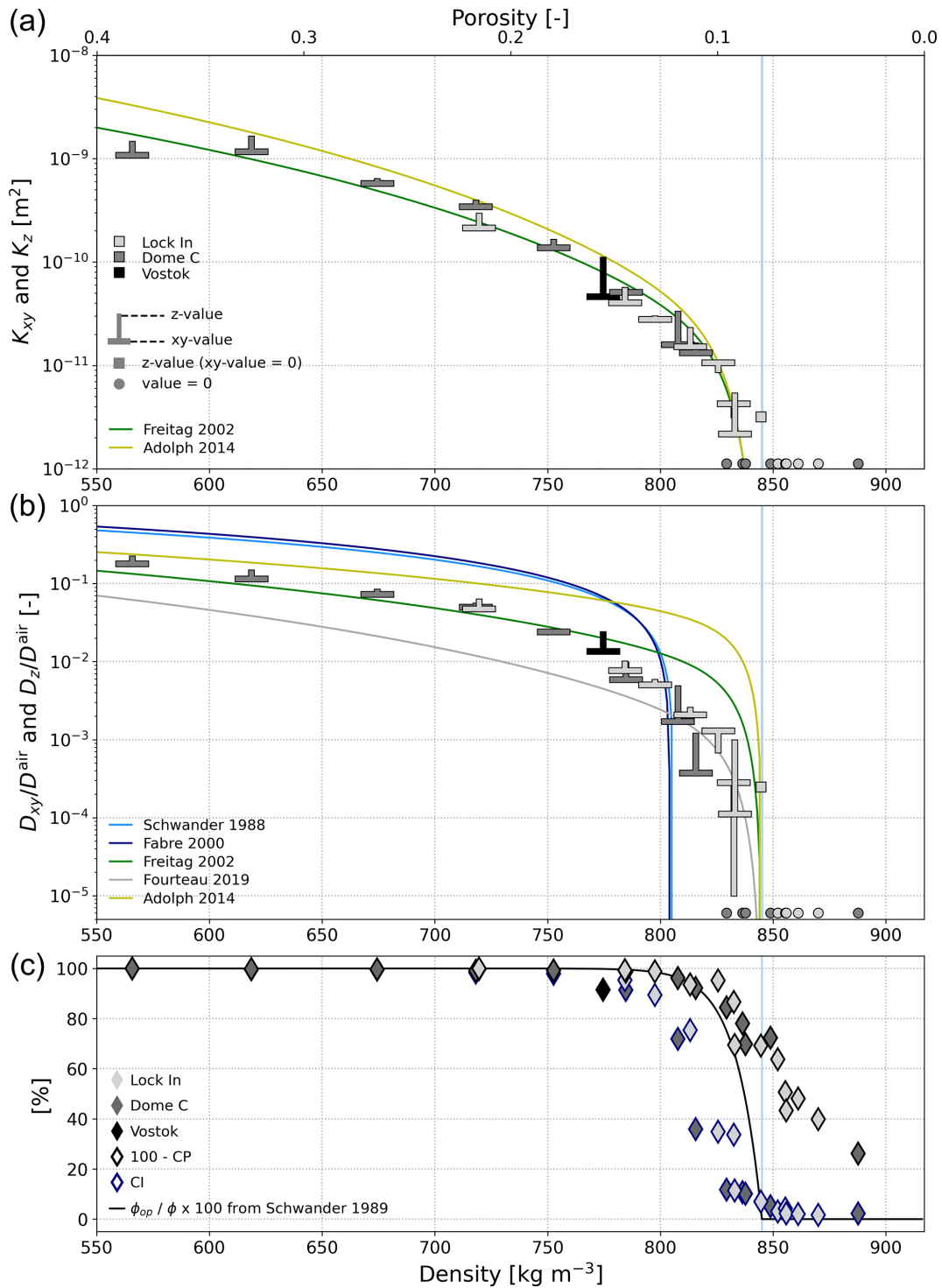
Figure 5. (a, b) Permeability and normalized diffusion coefficient of firm versus density: computations (“T” symbols) and regressions from the literature (lines). (c) Evolution with density of the open porosity fraction based on the closed-to-total porosity fraction CP and based on the open porosity from Schwander 1989, as well as the connectivity index CI. The vertical blue lines at 845 kg m -3 indicate the close-off density.
