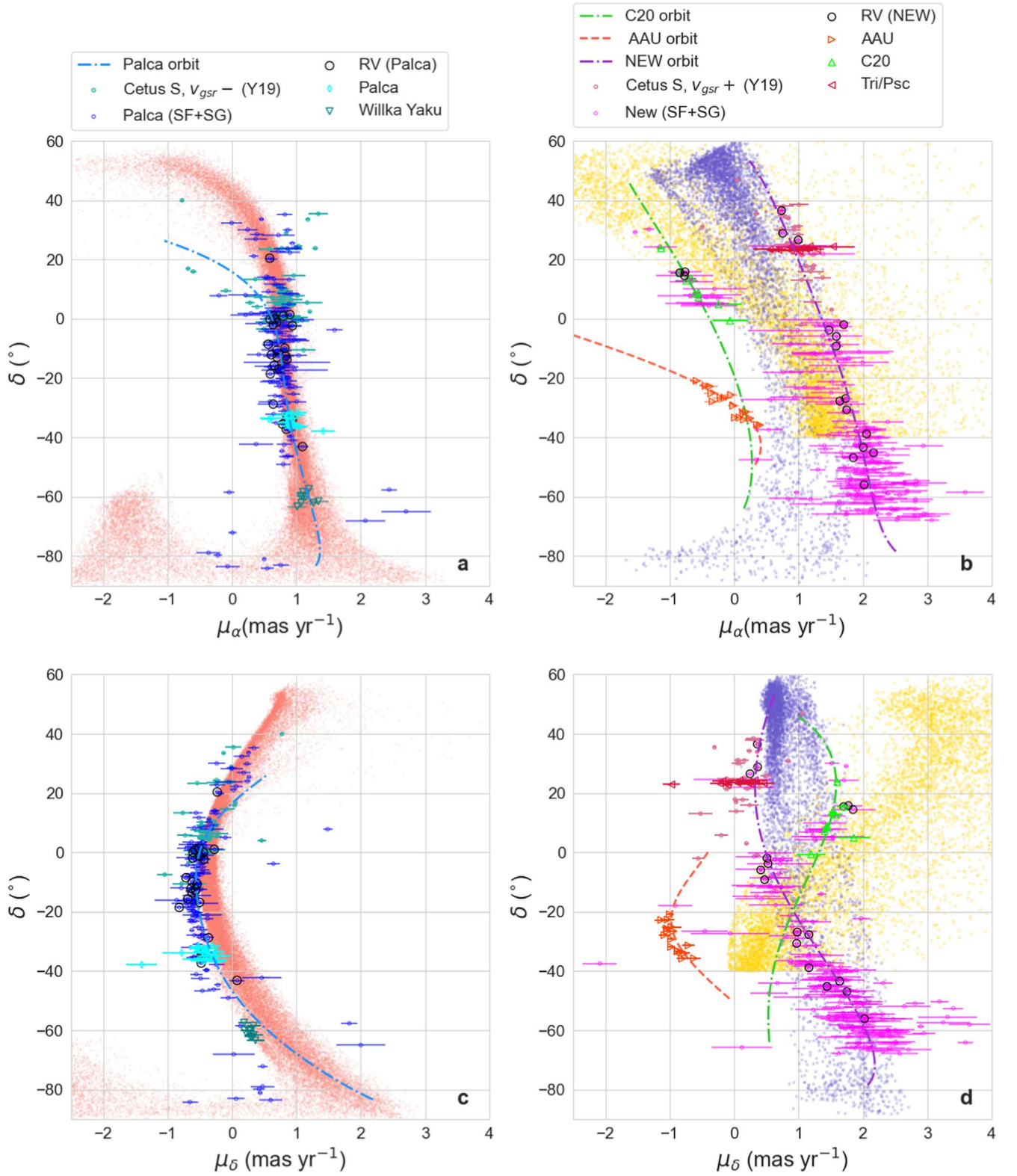
Figure 7. Same as Figure 6 in proper motion spaces, (\delta, \mu_{\alpha}) and (\delta, \mu_{\delta}) . (a) and (c) Cetus from Y19 (negative v_{\text{gsr}} , green), the Palca wrap detected in this work (blue), and the Palca (cyan diamonds) and Willka Yaku (dark green inverted triangles) streams from S5 (Li et al. 2021) form a continuous stream track, and agree with the averaged sampling orbit of the Palca wrap as well as T1 (orange). (b) and (d) Cetus (positive v_{\text{gsr}} , pink), the new southern wrap (magenta), and its orbit (purple), and the Tri/Psc stream (red left triangles) align with T2 (light purple). C-20 (light green) and its best-fitting orbit (green) generally agree with L1 (yellow), whereas AAU and its fitted orbit (orange) deviate further from L1.
