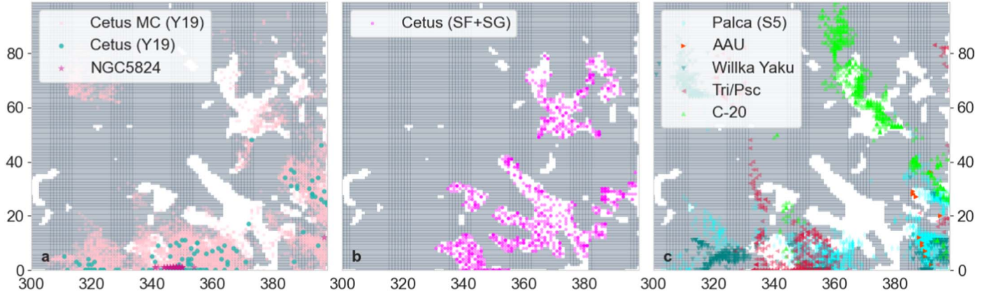
Figure 2. Zoom-in view of the SOM in the bottom-right corner of Figure 1, where the previous Cetus members from Y19 are mapped. The 130 Cetus members stars (green circles), all the MC realizations (100 for each) of the Cetus members (pink circles), and the MC realizations of NGC 5824 (violet star). (b) The DTGs are identified at u_{\text{thr}} = u_{30\%} in the Cetus region, and the stars from the STREAMFINDER sample associated with the Cetus DTGs are plotted by magenta circles. (c) The MC realizations of the 24 Palca members (cyan diamonds), 18 AAU members (orange right triangles), 11 Tri/Psc members (red left triangles), nine Willka Yaku members (dark green inverted triangles), and nine C-20 members (light green upper triangles) are mapped to SOM. Except for AAU, most of the realizations of the other stellar debris are located in the Cetus region.
