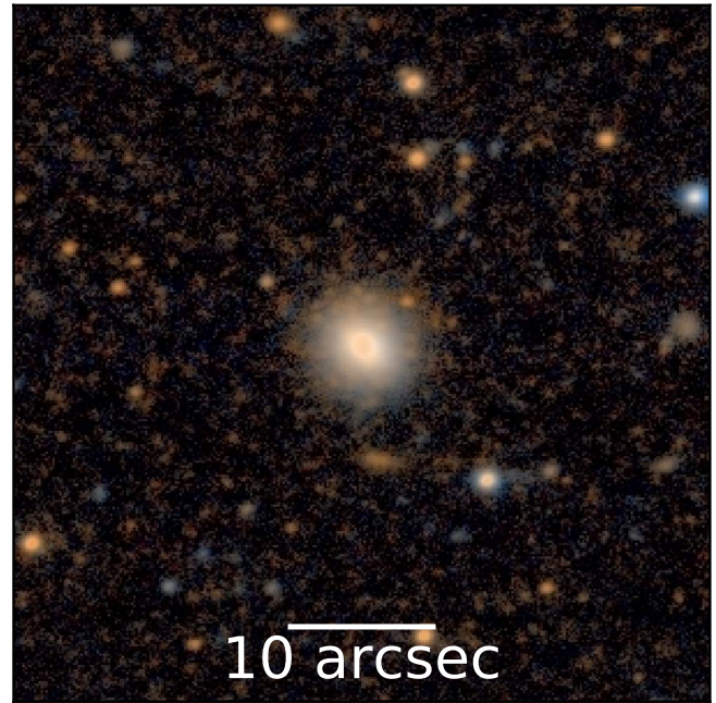
Figure 14. Color cutout of VHH81-01 from ground-based PISCeS imaging at the 6.5 m telescope Magellan Clay (Cmojević et al. 2016). The cutout is 0'.8 \times 0'.8 in size, and oriented such that north is up and east is left.
