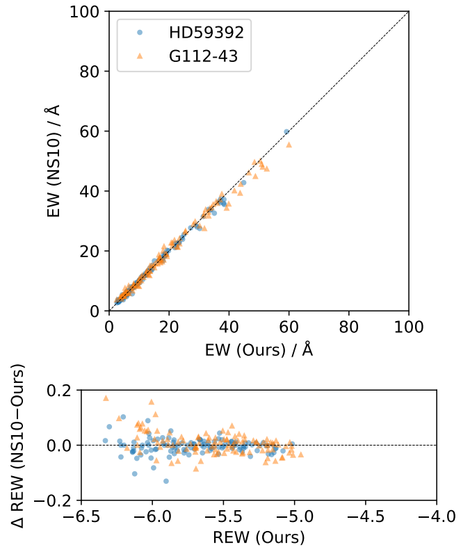
Fig. 2. Equivalent width comparison with NS 10.
