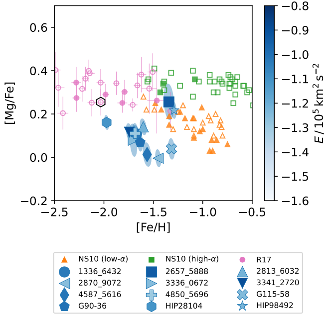
Fig. 5. Mg abundance of the stars. Kinematically selected Sequoia stars are plotted with blue symbols and color-coded according to their orbital energy (see Fig. 1). The measurement uncertainty and the covariance between [Mg/Fe] and [Fe/H] are indicated by the error ellipses. The data point circled with a black hexagon from R 17 indicates the abundance of HIP 28104. The abundance of the comparison samples comes from Nissen & Schuster (2010, 2011) , and Reggiani et al. (2017) . Filled symbols are for kinematically-selected Gaia-Enceladus stars among the comparison.
