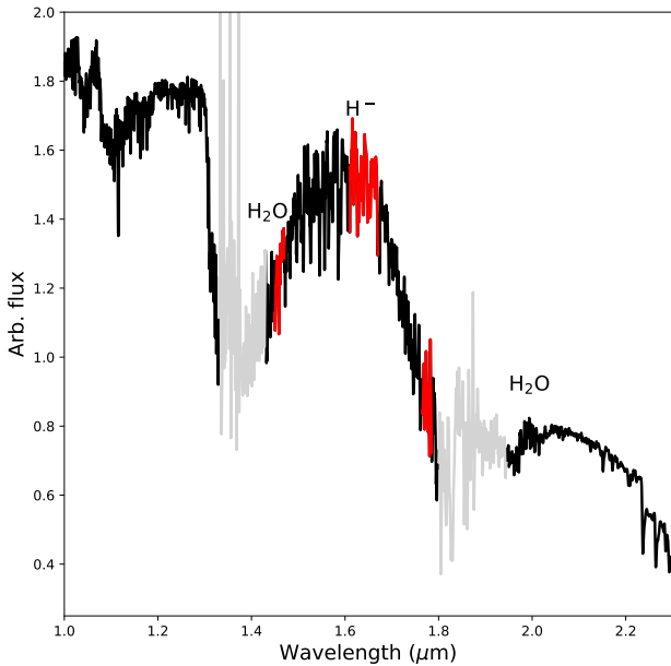
Fig. 3. Spectral H^-/H_2O feature. It is a combination of the 1.6\mu\text{m} ‘bump’ in the minimum opacity of H^- ion and H_2O vapour absorption bands around 1.4\mu\text{m} and 1.9\mu\text{m} . The index bands are marked in red. The telluric absorption is marked in grey. This spectrum is an average of O-rich TP-AGB stars with (I - K) = 3.19 .
