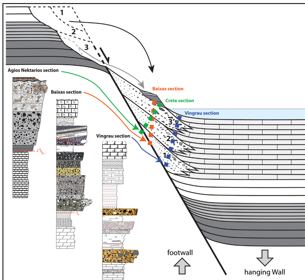
Figure 11. Sedimentological sections for southwestern Crete and the Bas Agly Basin positioned on an integrated model.
