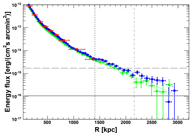
Fig. 5. Surface-brightness profiles of A 2142 obtained with different methods. The data points show the spectroscopic measurements (red), the azimuthally averaged profile (blue), and the azimuthal median (green). The green and blue thin dashed lines show the corresponding best fits obtained with the multiscale deprojection method. The solid and dashed horizontal lines correspond to the total background level and to the uncertainty on the background, respectively. The dashed and dash-dotted vertical lines represent R_{500} and R_{200} , respectively.
