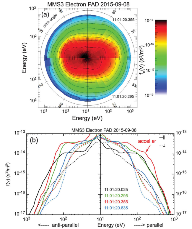
FIG. 4. Electron distributions from MMS3 near in time of the peak in E_{\parallel} and T_{e\parallel} . The origin is at the bulk electron velocity of each individual distribution. (a) Full pitch angle distributions 60 ms prior to the peaks (bottom—mirrored about the field direction for convenience) and closest to the peak (top). (b) Cuts parallel (solid) and perpendicular (dashed) to the magnetic field of the two distributions shown in (a)—green and red—along with cuts taken prior to the event and somewhat later—black and blue respectively. Times given in the plots are at the center of the 30 ms measurement interval.
