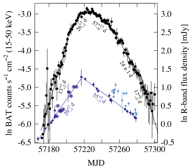
Figure 2. Swift /BAT (black circles) and dereddened optical R -band (blue diamonds; SMARTS data are encircled) light curves of the outburst overlaid. In addition, the e-folding times for the exponential rise and decay are marked for both outburst profiles. The light-blue diamonds are excluded in the calculation of the exponential decay in the R band.
