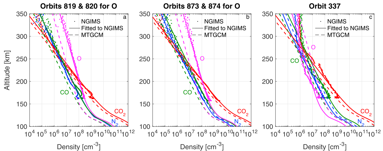
Figure B1. Neutral densities fitted to NGIMS (solid), NGIMS (dots), and MTGCM (dashed) are compared for (a) Orbit 819, (b) Orbit 873, and (c) Orbit 337. The CO 2 (red), CO (green), N 2 (blue), and O (magenta) are included in this model.
