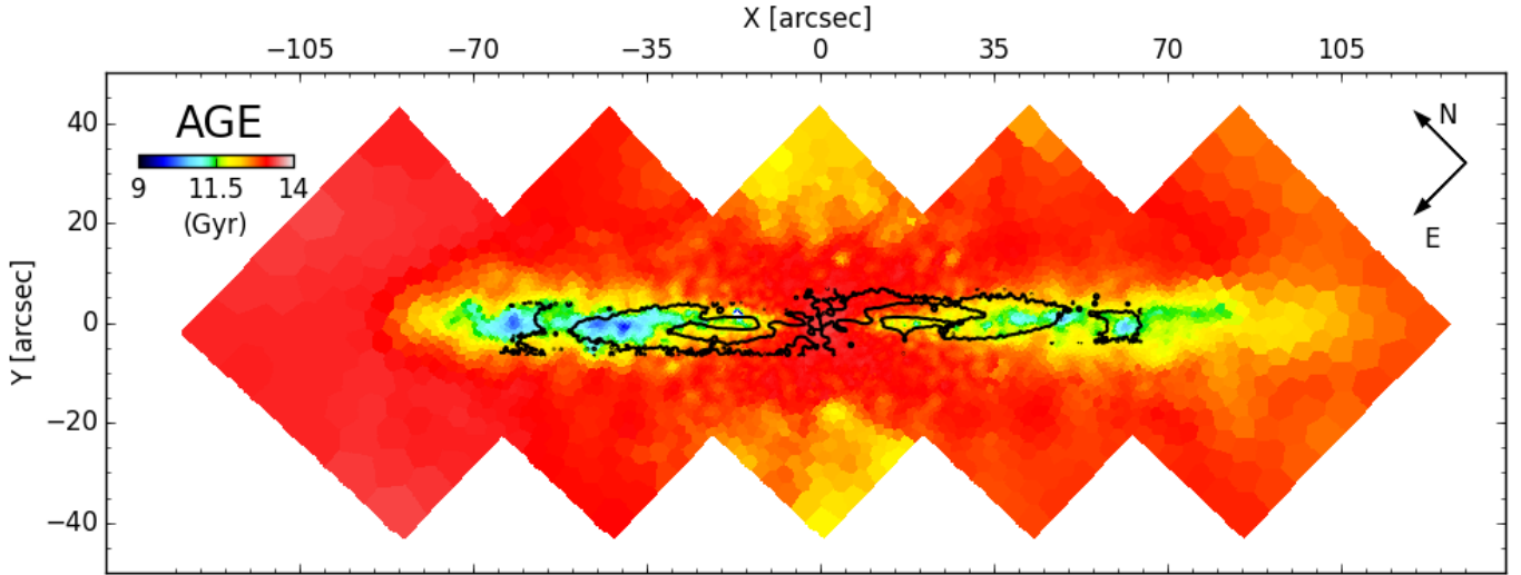
Fig. 12. Smoothed version of the stellar age map of NGC 3115; the ACS/HST residual contours are over-plotted. We plot only the zero-level contours corresponding to the potential spiral-arms in order to lighten their boundaries. A clear spatial match is observed between the spiral-like residual structures and the youngest stellar population observed.
