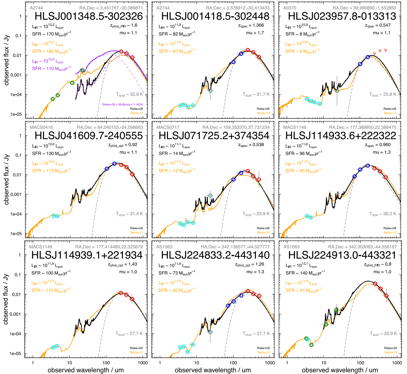
Figure 7. Example IR SEDs illustrating the observed photometry and fits. In each panel, observed (uncorrected) fluxes are shown by open circles: IRAC=cyan, MIPS=grey, WISE =green, PACS=blue, SPIRE=red. Non-detections ( 5\sigma upper limits) are denoted by a ‘v’. Also plotted are the best-fitting modified-blackbody (grey dashes), Rieke et al. (2009) template (black solid line) and Berta et al. (2013) template (orange solid line). Derived IR properties from each of the two template sets (in matching colours) take into account the magnification, \mu (shown to the right). Redshifts are spectroscopic ( z_{\text{spec}} ), optical photometric ( z_{\text{phot\_opt}} ) or IR-derived ( z_{\text{phot\_FIR}} ; see Section 4.4.1). For SEDs with a fitted AGN component, the two component model and star formation IR properties are shown in purple.
