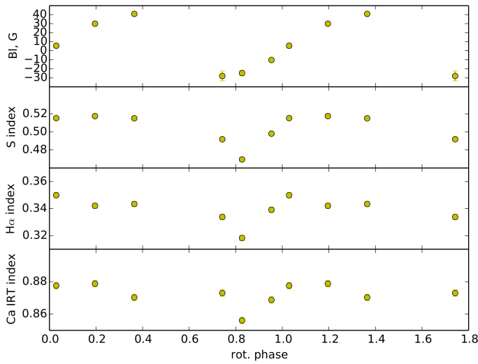
Fig. 6. B_l , S-index, H\alpha , Ca II IR triplet indexes behavior for observations of OU And gathered in 2008. The plots follow the same definitions as in Fig. 1.
