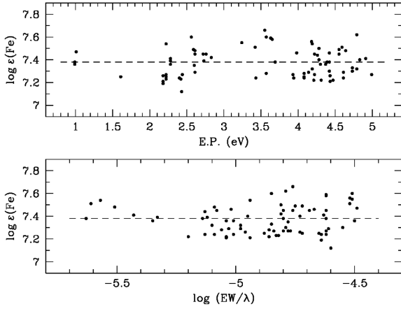
Fig. A.1. Abundance of Fe I lines versus excitation potential. The correct temperature is indicated by a zero slope in this plot. Bottom: abundance of Fe I lines versus showing determination of the microturbulent velocity.
