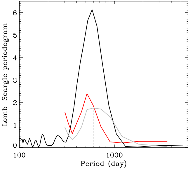
Fig. 3. Lomb-Scargle periodograms of the photometric activity proxy S_{\text{ph}} (black) and of the frequency shifts of the individual l = 0 (gray) and l = 1 (red) modes extracted from the analysis of KIC 10644253 using Method #2. Only independent points were used. The vertical dashed lines correspond to the associated maximum of the periodograms.
