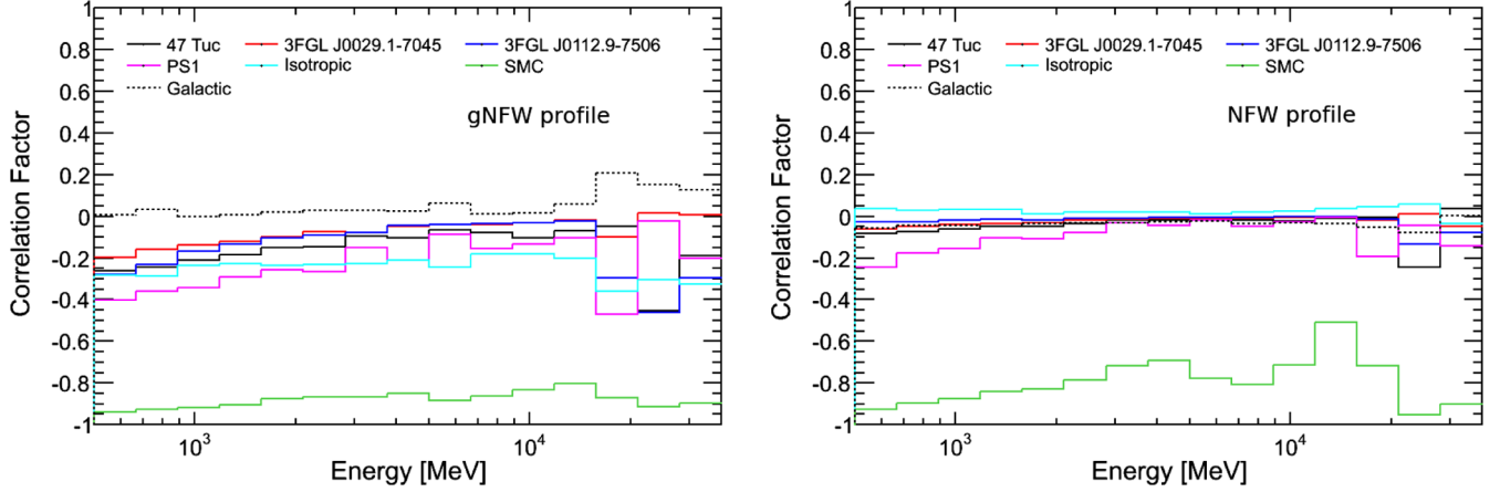
FIG. 4. Correlation factors, as given by Eq. (5), between the most important components of the background model and the two DM density profiles, g_{\text{NFW}} (left) and \text{NFW} (right), as a function of photon energy.
