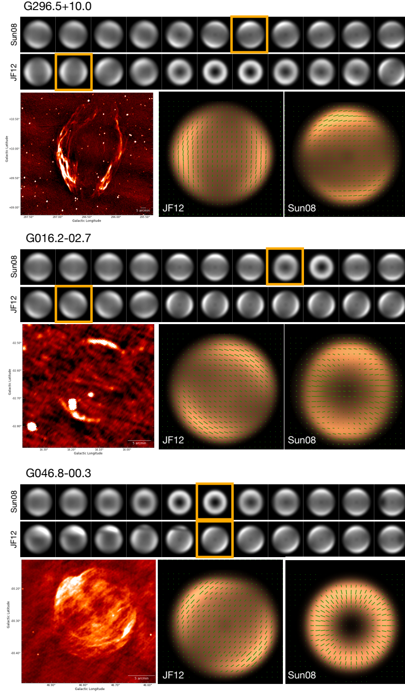
Fig. 7. Comparison of SNR models for three example SNRs: G296.5+10.0 (high-latitude), G016.2-02.7 (mid-latitude), and G046.8-0.3 (in the plane). All models from 0.5 to 10 kpc are shown (as described in Fig. D.1) for both GMF models: the Sun et al. (2008) (Sun08) and JF12. The orange box highlights the best fit in each case. Below the model strips we show the data ( left ) as well as the corresponding best fit model for JF12 ( center ) and Sun08 ( right ). The model polarization magnetic field vectors are overlaid in green.
