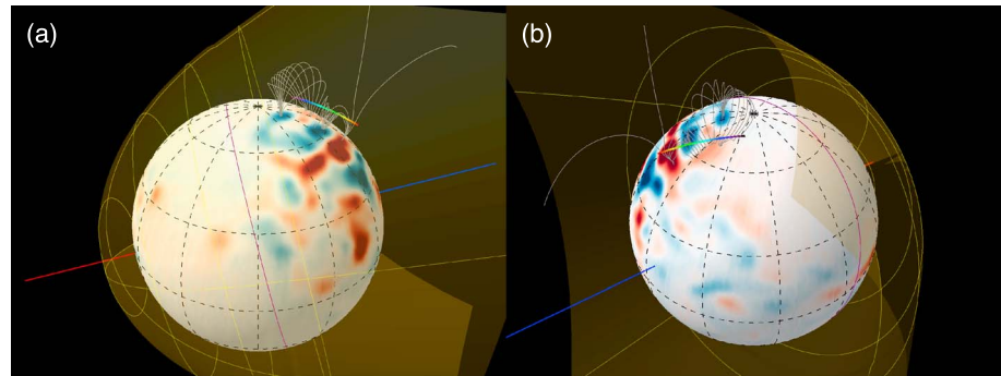
Figure 2. Three-dimensional (3-D) views of the field line topology (gray lines) [Morschhauser et al., 2014], nominal magnetic pileup boundary (yellow surface) [Trotignon et al., 2006], and MAVEN orbit (rainbow line) during the time interval shown in Figure 1. The radial component of the crustal magnetic field at ~400 km altitude [Connerney et al., 2001] is projected on the Mars surface ( R_M = 3389.9 km) with the linear color scale from -100 nT to +100 nT (the same color scale as Figure 3b). The red and blue bars indicate the Sun and anti-Sun directions, and the purple line on the surface denotes the day-night terminator. Note that these figures are viewed from the Southern Hemisphere and the South Pole is located on the upper side.
