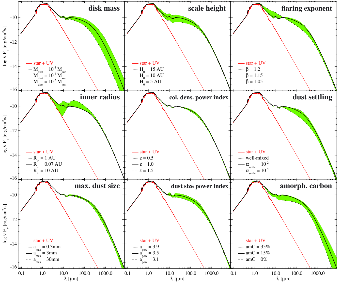
Fig. 8. Effect of dust and disk parameters on model SED at distance 140 pc and inclination 45°. The thick full black line is the reference model (identical in every part figure), whereas the green shaded area indicates the effect of a single parameter on the SED, where the dashed and dotted lines correspond to the changed parameter values as annotated. Top row: dust mass M_{\text{dust}} , scale height H_0 , and flaring exponent \beta . Second row: inner radius R_{\text{in}} , column density powerlaw index \epsilon , and dust settling parameter \alpha_{\text{settle}} . Third row: maximum grain size a_{\text{max}} , dust size powerlaw index a_{\text{pow}} , and volume ratio of amorphous carbon. The dependencies of the SED on the tapering-off radius R_{\text{tap}} (not shown), on the outer radius R_{\text{out}} (not shown), and on the minimum dust particle size a_{\text{min}} (not shown) are less than the one shown for \epsilon .
