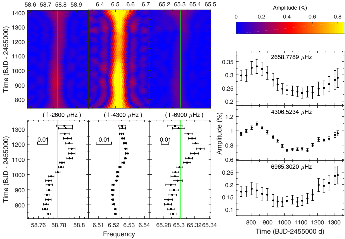
Fig. 12. Frequency and amplitude modulations of the components that form the linear combination f_{1-} + f_4 = f_8 . The panels are similar to those described in Fig. 7. The three components show clear periodic modulations evolving in phase. In each bottom left subpanels , a segment indicates the 0.01 \mu\text{Hz} scale.
