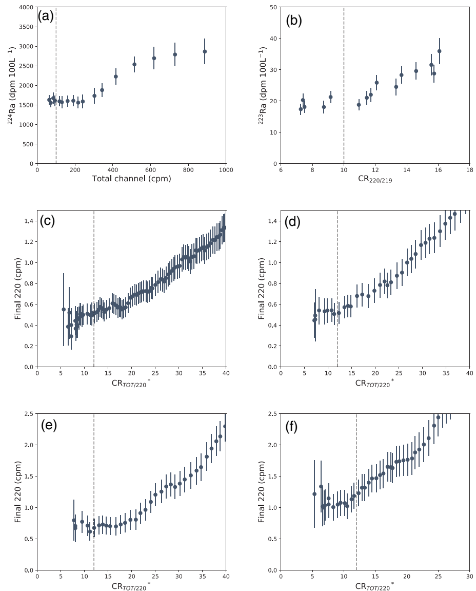
Figure 9. Compilation of measurements performed in the UAB laboratory. (a) Quantification of ^{223}\text{Ra} (b) and ^{224}\text{Ra} (a) against Total channel count rate and \text{CR}_{220/219} , respectively, from the repeated measurement of a high activity ^{223}\text{Ra} and ^{224}\text{Ra} sample (20 and 1,600 dpm 100 L ^{-1} , respectively). The Final220 count rate is evaluated in function of the Total channel count rate for four different measurements (c)–(f). The dashed lines indicate the quantification limits in cases of (a) high activity measurements, (b) 219–220 cross-talk effect, and (c–f) ^{222}\text{Rn} buildup effect.
