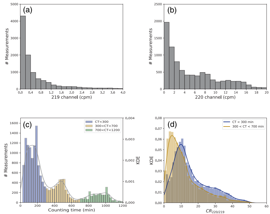
Figure 2. Histogram (a, b, and c) and kernel density estimate (KDE) (c and d) of 16,906 measurements performed by eight different laboratories between 2004 and 2018. (a) Count rate in the 219 channel ( 30 < CT < 800 min). (b) Count rate in the 220 channel ( 30 < CT < 300 min and CR_{220/219} > 1 ). (c) Counting times. (d) CR_{220/219} . Blue, yellow, and green colors indicate counting times of CT < 300 , 300 < CT < 700 , and 700 < CT < 1200 min, respectively.
