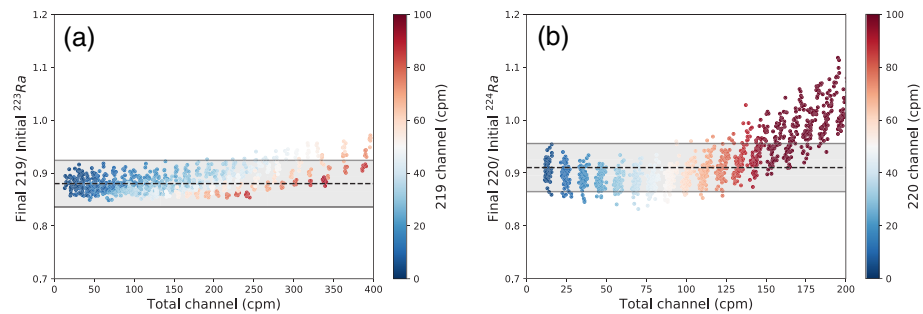
Figure 4. Results from simulations ( n = 2,290 ) with initial ^{223}\text{Ra} , ^{224}\text{Ra} , and ^{226}\text{Ra} count rates ranging 0–100, 0–100, and 0–25 cpm, respectively. (a) Ratio between corrected 219 channel and initial ^{223}\text{Ra} simulated count rates ( \text{Final219}/\text{Initial}^{223}\text{Ra} ) against Total channel count rate. (b) Ratio \text{Final220}/\text{Initial}^{224}\text{Ra} against Total channel count rate. The dashed line represents the gate efficiency ( f_G ) and the gray band an uncertainty of 5%. The color scale represents the count rate in the Total channel.
