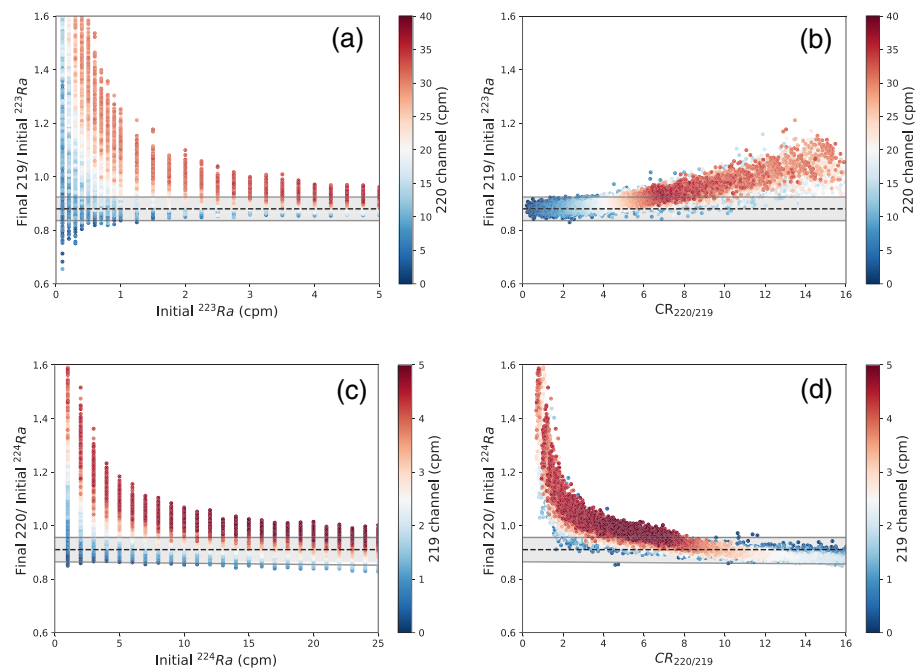
Figure 5. Results from simulations ( n = 18,250 ) with initial ^{223}Ra , ^{224}Ra , and ^{226}Ra count rates ranging 0–5, 0–25, and 0–25 cpm, respectively. The ratio between corrected 219 channel and initial ^{223}Ra simulated count rates ( Final219/Initial^{223}Ra ) against (a) Initial^{223}Ra and (b) CR_{220/219} . The ratio Final220/Initial^{224}Ra against (c) Initial^{224}Ra and (d) CR_{220/219} . Colors represent the 219 (a and b) and 220 (c and d) channels count rate. The dashed line represents the gate efficiency ( f_G ) and the gray band an uncertainty of 5%. Solid lines indicate the CR_{220/219} limits for quantification.
