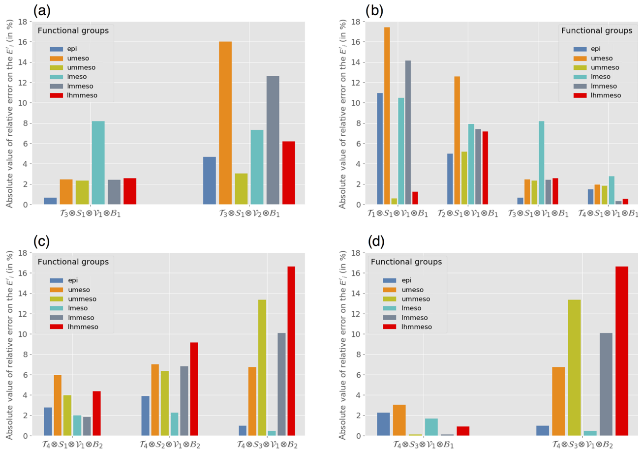
Figure 3. Mean relative error ( E_i in %, Eq. 9) on each E_i coefficients for (a) Exp. 1c and d, which present the following tested regimes: high versus low velocities in temperate temperatures, weak-stratification regimes and bloom regimes; (b) Exp. 2a, 2b, 2c and 2d, which compares polar, subpolar, temperate and tropical temperatures in weak-stratification, low-velocity and bloom regimes; (c) Exp. 3a, b and c, which compares weak, intermediate and high stratification in tropical-temperature, low-velocity and no-bloom regimes; and (d) Exp. 4c and d: bloom versus no-bloom regimes in tropical temperatures, strong stratification and low velocities.
