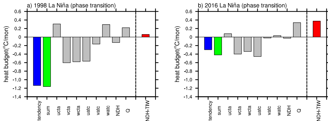
FIG. 7. Comparison of the mixed layer SST heat budget analysis over the TIW active region (5°S–5°N, 110°–150°W) (units: ^{\circ}\text{C month}^{-1} ) during the ENSO phase transition (May–June) of (a) 1998 and (b) 2016. Here “sum” (green bar) means the summation of all terms on the right side of Eq. (4). The bars, from left to right, indicate the mixed layer temperature tendency, sum of all terms on the right-hand side of Eq. (4), the anomalous zonal and meridional advection terms [-\tilde{u}(\partial \tilde{T}/\partial x) and -\tilde{v}(\partial \tilde{T}/\partial y) ], anomalous upwelling advection term [-\tilde{w}(\partial \tilde{T}/\partial z)] , mean horizontal advection terms [-\bar{u}(\partial \tilde{T}/\partial x) and -\bar{v}(\partial \tilde{T}/\partial y) ], mean upwelling advection term [-\bar{w}(\partial \tilde{T}/\partial z)] , low-order NDH associated with the low-frequency ( >60 days) variability [\bar{u}(\partial \tilde{T}/\partial x) + \bar{v}(\partial \tilde{T}/\partial y) + \bar{w}(\partial \tilde{T}/\partial z)] , the atmospheric heat flux ( Q ), and TIW-induced NDH ( \text{NDH}_{\text{TIW}} ).
