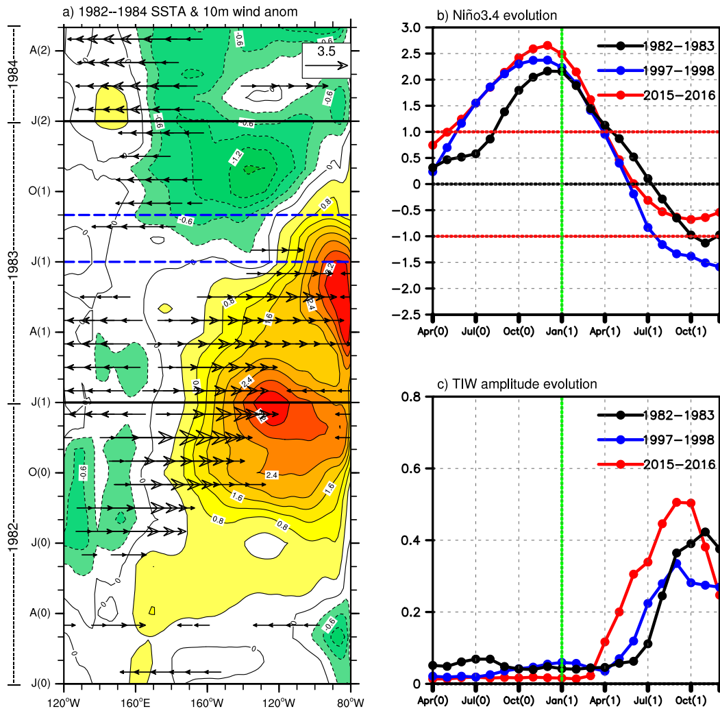
FIG. 12. (a) The shading shows the evolution of equatorial SST anomalies ( ^{\circ}\text{C} ) and the vector field shows the anomalous 10-m zonal wind ( \text{m s}^{-1} ) averaged over 5^{\circ}\text{S} – 5^{\circ}\text{N} for the 1982/83 event. (b) Time evolution of SST anomalies for the El Niño/La Niña events of 1982/83 (black), 1997/98 (blue), and 2015/16 (red) in the Niño-3.4 region ( 5^{\circ}\text{N} – 5^{\circ}\text{S} , 120^{\circ} – 170^{\circ}\text{W} ). (c) Time evolution of TIW amplitude of 1982/83 (black), 1997/98 (blue) and 2015/16 (red).
