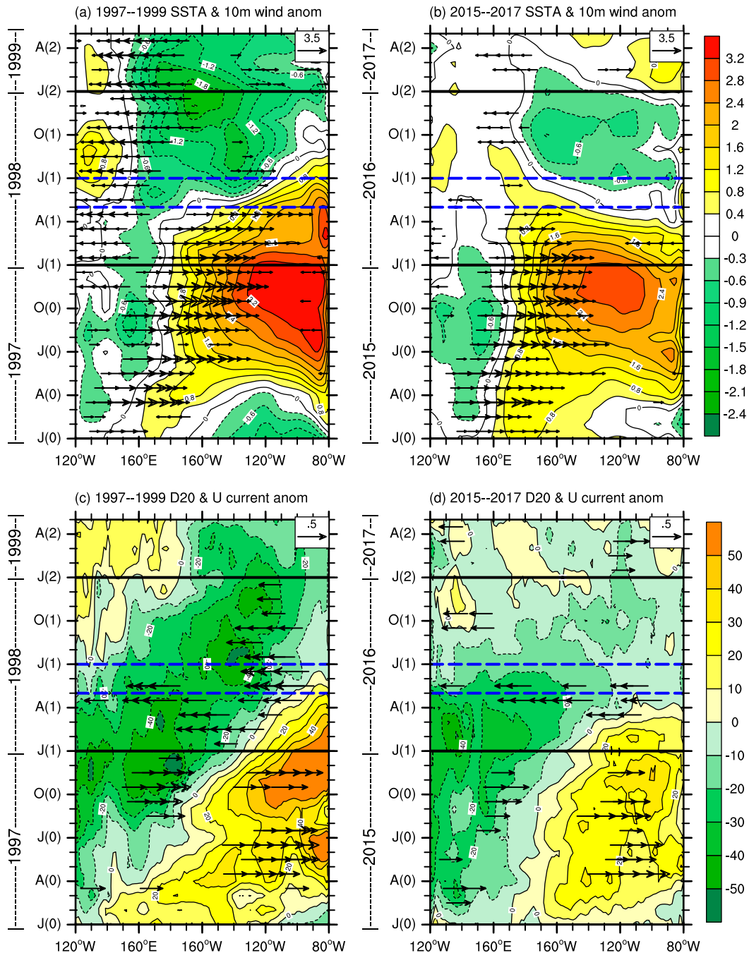
FIG. 3. The shading shows the evolution of equatorial SSTA ( ^{\circ}\text{C} ) and the vector fields show the anomalous 10-m zonal wind ( \text{m s}^{-1} ) averaged over 5^{\circ}\text{S} – 5^{\circ}\text{N} for (a) the 1997/98 event and (b) the 2015/16 event. (c),(d) As in (a) and (b), but for the evolution of the equatorial 20^{\circ}\text{C} thermocline depth (D20) anomalies and oceanic surface zonal current anomalies. The number 0 in parentheses denotes the ENSO developing year (1997 and 2015), the number 1 denotes the El Niño decaying year (1998 and 2016), and the number 2 denotes the following year (1999 and 2017). The legend at the upper-right corner of each panel indicates a reference vector magnitude.
