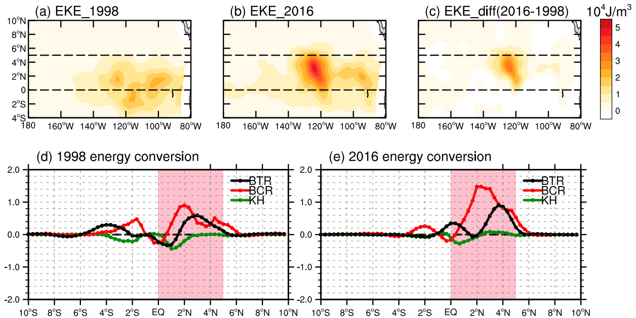
FIG. 8. Maps of mean TIW EKE (units: 10^4 \text{ J m}^{-3} ) over the TIW region ( 4^{\circ}\text{S} – 10^{\circ}\text{N} , 180^{\circ} – 80^{\circ}\text{W} ) during the ENSO phase transition of (a) 1998 and (b) 2016, and (c) their difference. (d),(e) Zonally averaged energy conversion (units: 10^5 \text{ W m}^{-3} ) over the Niño-3 region ( 90^{\circ} – 150^{\circ}\text{W} ) between EKE and the mean kinetic energy (black dotted line), available potential energy (red dotted line), and Kelvin–Helmholtz energy conversion (green dotted line) for 1998 and 2016, respectively.
