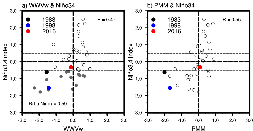
FIG. 13. Scatterplots of the relationship between ENSO amplitude (Niño-3.4 index: 5^{\circ}\text{S} – 5^{\circ}\text{N} , 170^{\circ}\text{W} – 90^{\circ}\text{W} ) at its peak (NDJ) between (a) WWVw ( 5^{\circ}\text{S} – 5^{\circ}\text{N} , 120^{\circ}\text{E} – 155^{\circ}\text{W} ) 13 months before (i.e., \text{OND}_{\text{Year}(-1)} ) (b) and monthly mean PMM wind index during ENSO transition phase (May–June) from 1980 to 2018. The coefficients ( R ) are labeled in the upper-right corner of the corresponding panel. The coefficient ( R ) between WWVw and Niño-3.4 index during La Niña years is labeled in the lower-left corner of the corresponding panel.
