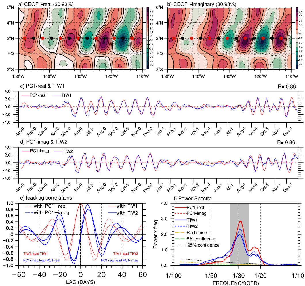
FIG. 2. (a),(b) Leading CEOF spatial patterns of SSTAs over the TIW active region ( 2^{\circ}\text{S} – 6^{\circ}\text{N} , 110^{\circ} – 150^{\circ}\text{W} ) over the 2016–17 period [for the (a) real and (b) imaginary parts] obtained through a linear regression of SSTAs onto the normalized real part (PC1-real) and imaginary part (PC1-imag) of the leading PC time series. Red (black) dots show the positions of longitudinal nodes used to calculate TIW1 (TIW2). (c),(d) Corresponding normalized PC time series of leading CEOF mode (red lines) and complex TIW index (blue lines), respectively. Number 0 in parentheses denotes the year 2016, and the number 1 denotes the following year (2017). All results are statistically significant above the 99% confidence level. (e) Lead–lag correlations between TIW1 and TIW2 (solid blue line) and TIW1 autocorrelation (solid red line), and the same for the PCs (dashed lines and similar color code). (f) Power spectra of the normalized PC1 (red line) and TIW index time series (blue line); solid (dashed) lines are for the real (imaginary) part. The plotting format forces the area under the power curve to be equal to the variance in any frequency band. The gray bar indicates the approximate TIW frequency peak. The dashed orange line is the red-noise spectrum inferred from a first-order autoregressive process. The 5% (95%) confidence intervals are shown by the dashed green (black) lines.
