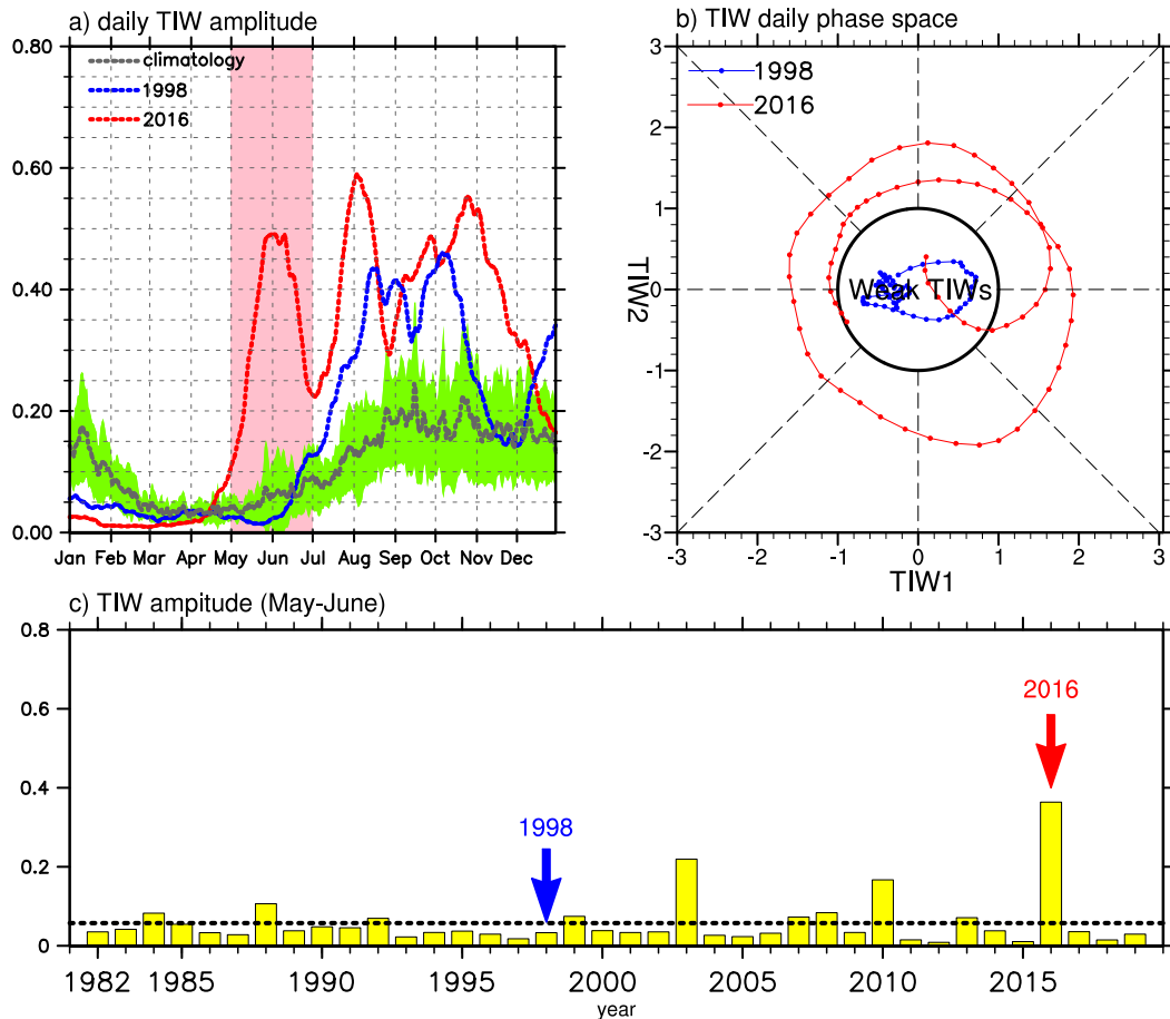
FIG. 4. (a) Time series of the daily TIW amplitude for the 1998 (blue), the 2016 La Niña event (red), and the climatology (gray). The green shades represent one standard deviation error estimates. (b) (TIW1, TIW2) phase-space points for all available days during May–June for 1998 (blue) and 2016 (red). The region of weak TIW activity is labeled. (c) Annual TIW amplitude (May–June) during 1982–2018 (yellow bars) and the corresponding climatological mean state during ENSO phase transition (black dashed line).
