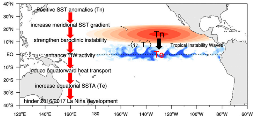
FIG. 11. Schematic diagram illustrating the dynamical mechanism responsible for hindering the 2016 La Niña development through the equatorward heat transport from the strong TIW activity.
