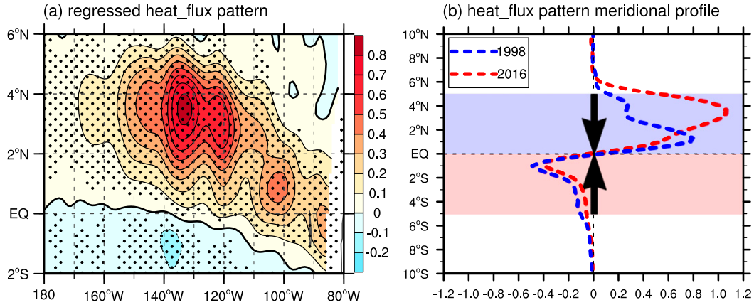
FIG. 6. (a) TIW-induced meridional heat flux regressed onto the standardized monthly TIW amplitude for all months during 1980–2018. Values exceeding the 99% confidence level are marked by black dots. (b) The blue line and red line denote the meridional structures of zonal mean (110°–150°W) heat flux pattern (units: 10^5 \text{ m}^2 \text{ C}^{-1} \text{ month}^{-1} ) during ENSO phase transition (May–June) for 1998 and 2016, respectively. The black arrows indicate the eddy heat flux convergence.
