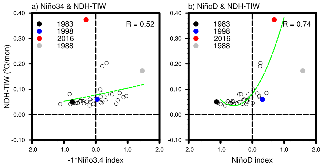
FIG. 10. Scatterplots of the relationship of the monthly mean (a) Niño-3.4 index and (b) NiñoD index, respectively, with the reconstructed TIW-induced NDH during the ENSO transition phase (May–June) from 1982 to 2018. The green lines indicate the nonlinear regression lines and the nonlinear correlation coefficients ( R ) are labeled in the upper-right corner of the corresponding panel.
