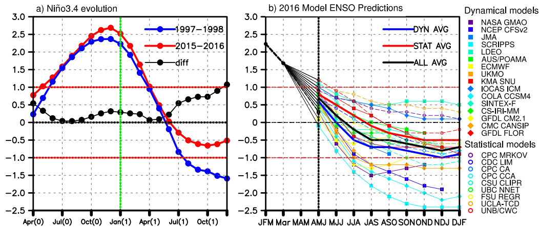
FIG. 1. (a) Time evolution of SST anomalies in the Niño-3.4 region ( 5^{\circ}\text{N} – 5^{\circ}\text{S} , 120^{\circ} – 170^{\circ}\text{W} ) for the El Niño/La Niña events of 1997/98 (blue) and 2015/16 (red), and their difference (black). (b) Plume of forecasts of the Niño-3.4 SST anomaly from dynamical and statistical models that were run in mid-April 2016. The average of the forecasts of the dynamical models is shown by the thick blue line, and of the statistical models by the thick red line. The average of all the models is shown by the thick black line.
