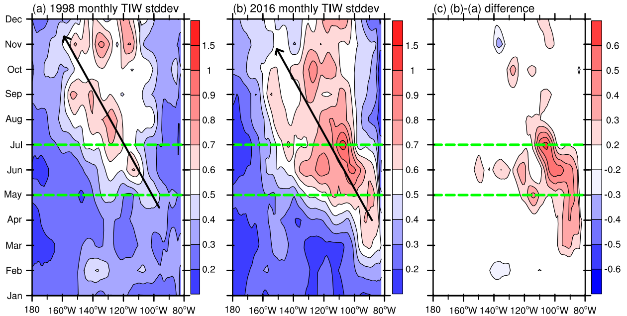
FIG. 5. Longitude–time diagrams of monthly TIW standard deviations averaged over 0^{\circ} – 6^{\circ} N for (a) 1998 and (b) 2016, and (c) their difference.
