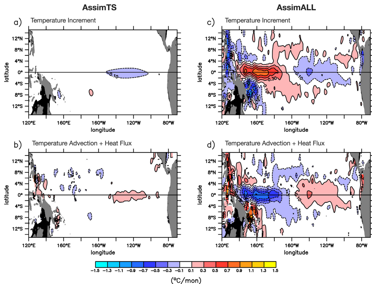
Fig. 12. (a) Mean temperature increment averaged in the 0–300 m layer and (b) the mean advection and heat flux terms of Eq. (2) from AssimTS. (c,d) Same as (a,b) except for AssimALL.
