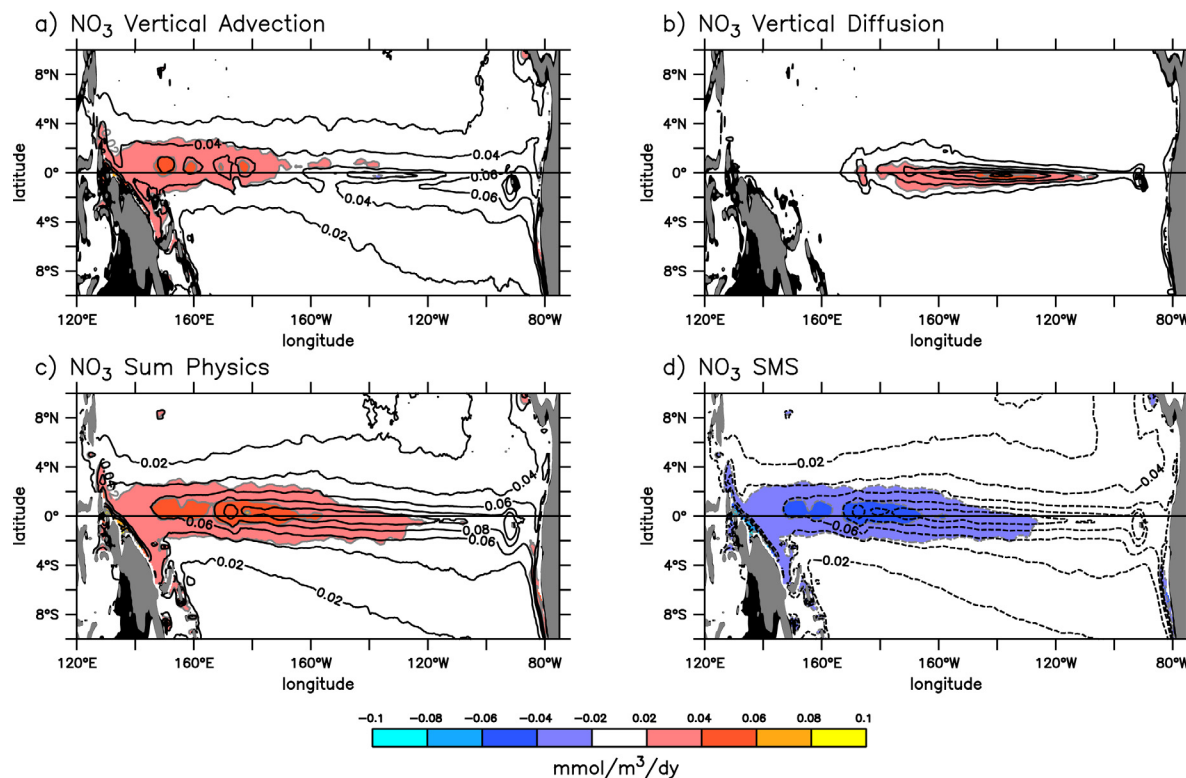
Fig. 2. (a) Map of the 2008–2014 mean of the vertical advection flux of nitrate averaged in the euphotic layer from AssimALL (contours) and the difference from AssimTS (color shading). (b) Same as (a) but for the vertical diffusion flux of nitrate. (c) Same as (a) except for the sum of the fluxes from physics processes (horizontal advection, vertical advection, vertical diffusion). (d) Same as (a) except for the fluxes from biological processes (SMS = source minus sink). Unit is \text{mmol}/\text{m}^3/\text{dy} .
