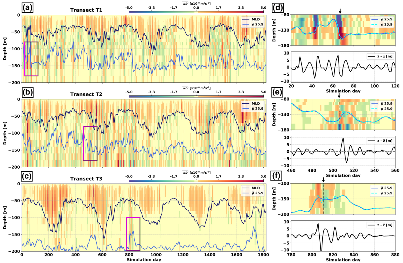
Figure 5. Left: model timeseries of the along-transect averaged SBF ( \overline{wb'} ) for T1 (a), T2 (b), and T3 (c). The dark blue line represents the MLD, and the light blue line represents the \bar{\rho} = 1025.9 \text{ kg m}^{-3} isopycnal. The magenta boxes indicate periods of strong SBF events affecting \bar{\rho} . Right: blowout of strong SBF events within the model timeseries for T1 (d), T2 (e), and T3 (f). The cyan line represents the \rho = 1,025.9 \text{ kg m}^{-3} isopycnal. The blue line represents the 6-day mean \bar{\rho} = 1025.9 \text{ kg m}^{-3} isopycnal. The black line in the lower panels represents the depth difference between the isopycnal \rho and the mean isopycnal \bar{\rho} . The arrow and dashed line indicate 1 day of simulation with strong SBF.
