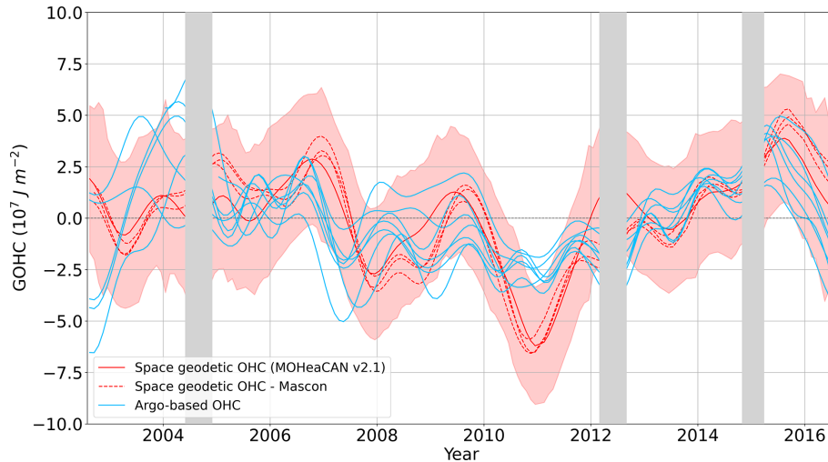
Figure 5. Interannual variations in global ocean heat content (GOHC) change. A 13-month low-pass filter is applied after removing periodic signals (annual and semi-annual) and trend. Red lines correspond to space geodetic estimates where estimates based on mascon ocean mass are represented as dashed lines and MOHeaCAN v2.1 is represented by the mean value (solid red) and the uncertainty at 1-sigma (shaded areas). Blue lines correspond to the Argo-based estimates from 2005. Grey areas correspond to the data gaps in the gravimetry product used for the space geodetic GOHC change.
