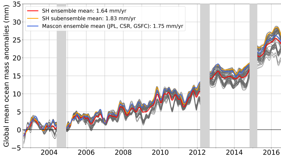
Figure A1. Comparison of global mean ocean mass changes from satellite gravimetry based on spherical harmonics solutions (LEGOS ensemble V1.4, in grey) and mascon solutions over August 2002–August 2016 for the global ocean. The mean of the full spherical harmonic ensemble is shown in red. The mean of the spherical harmonic ensemble subset consistent with mascons is shown in orange. The mean of the three mascon solutions considered in this study is shown in blue.
