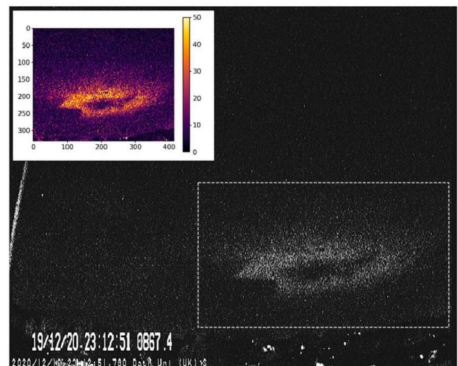
Fig. 7. The first ever elve detected from the UK on a low-light camera installed at the University of Bath. The CG stroke ( -750 kA) responsible of this optical emission on the lower ionosphere was located close to the NW coast of France ( \sim 400 km from the camera).
