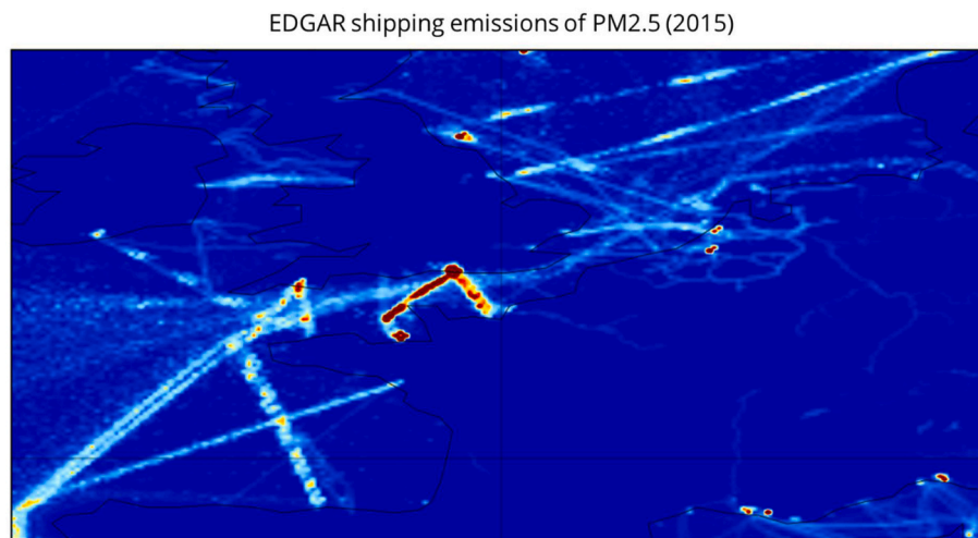
Fig. 16. Map of shipping emissions in the study area using data from EDGAR (Emissions Database for Global Atmospheric Research) for the year 2015, showing the largest concentrations of PM_{2.5} particles on the English Channel.
