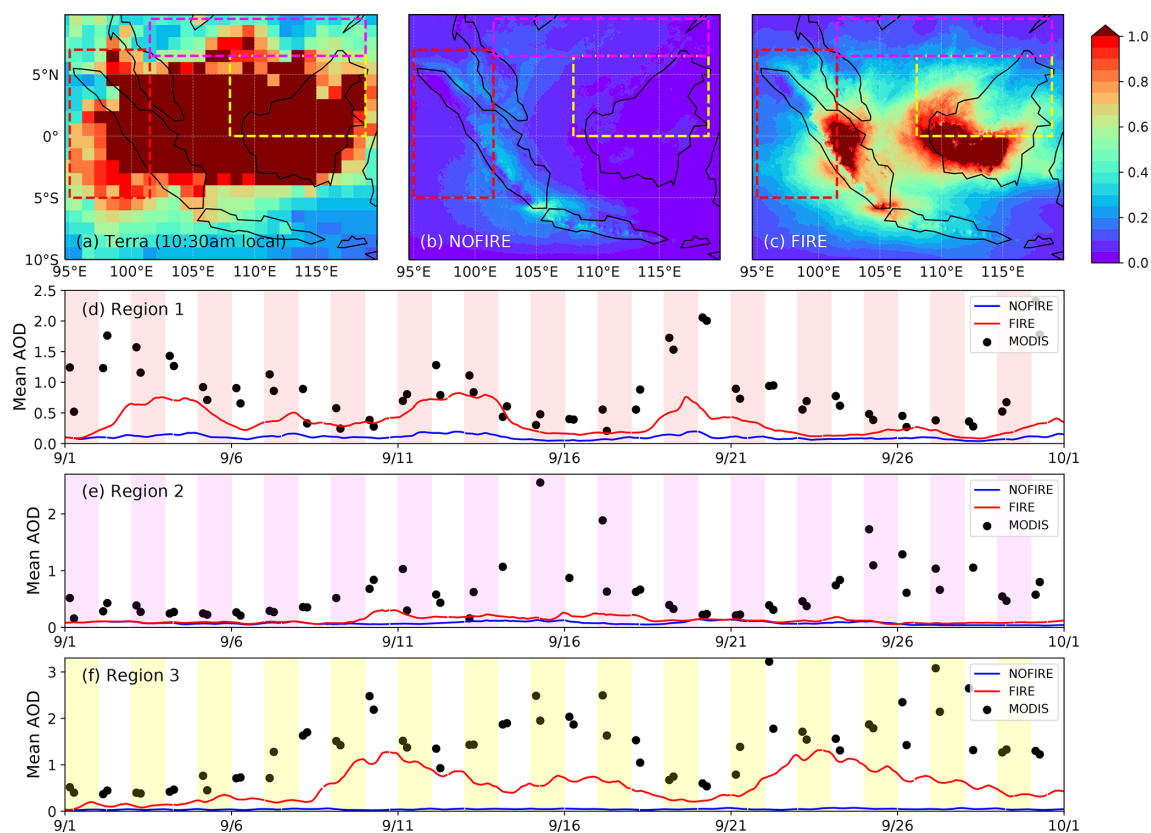
Figure 6. Monthly mean AOD at 0.55\ \mu\text{m} (a) observed by MODIS Terra (MOD08_D3) and (b) simulated in NOFIRE and (c) FIRE. AOD from MODIS Aqua (MYD08_D3) shows a similar result. The simulated results in (b) and (c) are the averages of AOD snapshots at 03:20 UTC every day, which corresponds to 10:20 Indochina time. Time series of observed (black dots, twice daily) and simulated (blue and red lines, hourly) AODs averaged over each region are shown for (d) Region 1, (e) Region 2, and (f) Region 3. In (d)–(f), both Terra and Aqua are included. Note that the MODIS data were projected onto the UTC time series in (d)–(f), assuming that the data were taken at 10:30 and 13:30 Indochina time.
