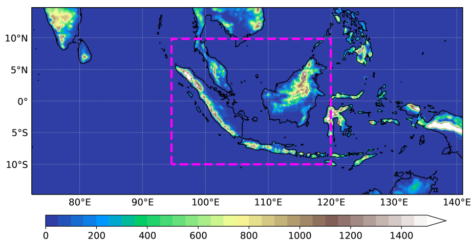
Figure 4. Terrain height (m) within the outer simulation domain, which is outlined by the map. The inner domain is outlined by the magenta rectangle.
