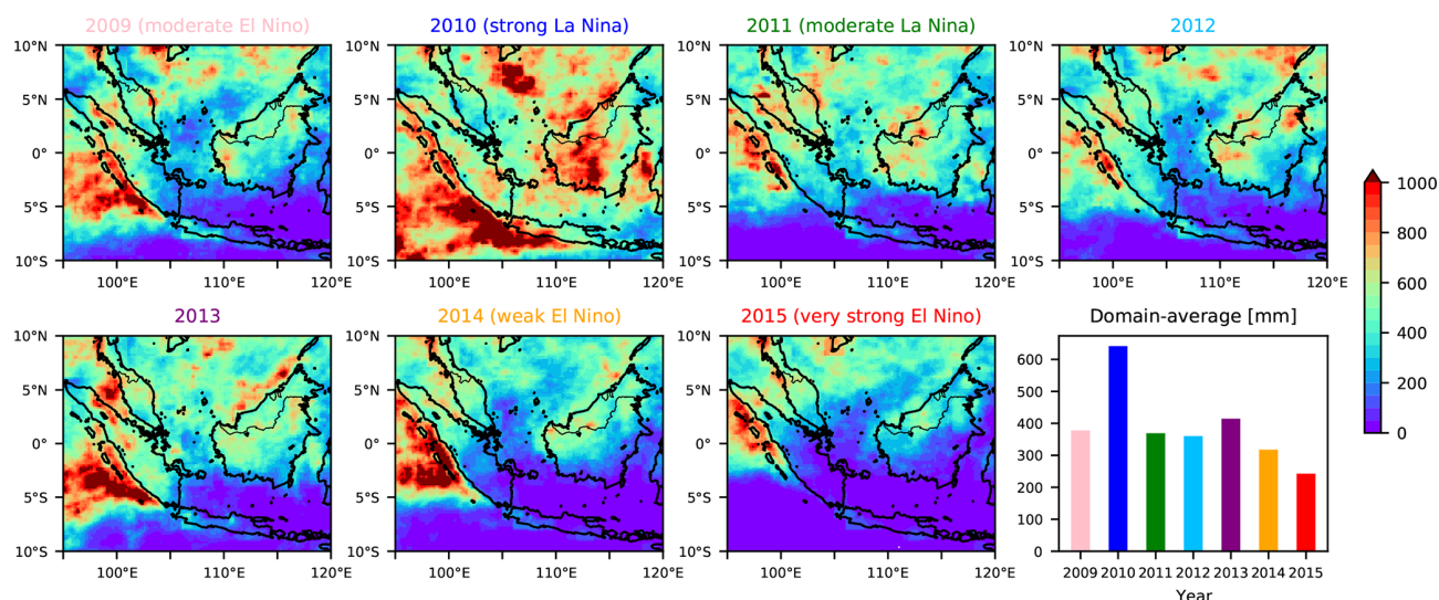
Figure 1. The 2-month accumulated precipitation (mm) observed by TRMM in September and October of each year from 2009 to 2015, calculated from the monthly mean precipitation rate data (TRMM 3B43). Domain-mean amounts are shown in the bar graph at lower right. The ENSO phases are based on the 3-month running mean Oceanic Niño Index ( https://origin.cpc.ncep.noaa.gov/products/analysis_monitoring/ensostuff/ONI_v5.php , last access: 25 March 2022).
