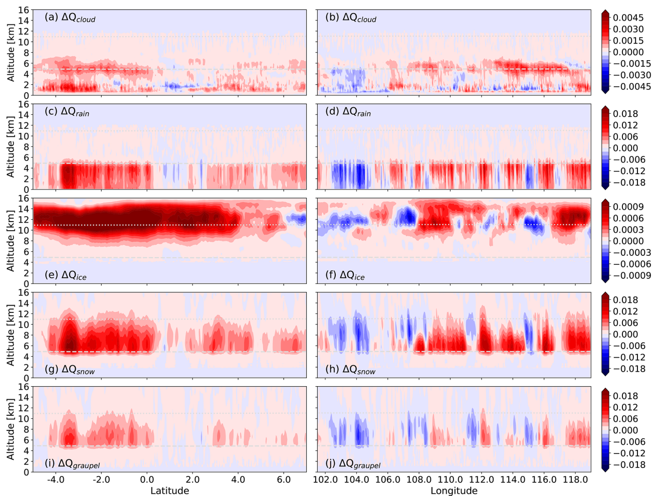
Figure A1. Same as (c, f, i, l, o) in Fig. 11 but for (a, c, e, g, i) Region 1 and (b, d, f, h, j) Region 2. Note that it is a zonal mean, rather than a meridional mean, for Region 1.
