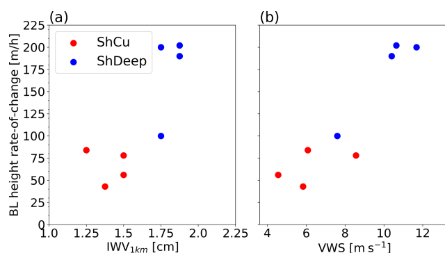
Figure 9. Scatterplots of the BL height rate of change versus (a) integrated water vapor from 50 to 1000 m ( IWV_{1km} ) and (b) vertical wind shear (VWS) between 50 and 1000 m for shallow-to-deep convective (ShDeep, blue circles) and shallow convective (ShCu, red circles) days.
