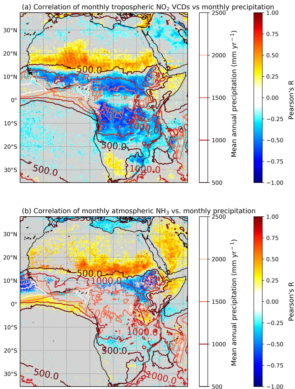
Figure 2. Relationship between monthly precipitation and monthly nitrogen dioxide (NO 2 ) (2005–2017) or ammonia (NH 3 ) vertical column densities (VCDs) (2008–2017). Per grid cell correlation coefficients between mean monthly precipitation and (a) tropospheric NO 2 VCDs and (b) atmospheric NH 3 VCDs overlaid with mean annual precipitation isolines. Gray areas indicate region with insignificant correlation ( p > 0.05 ).
