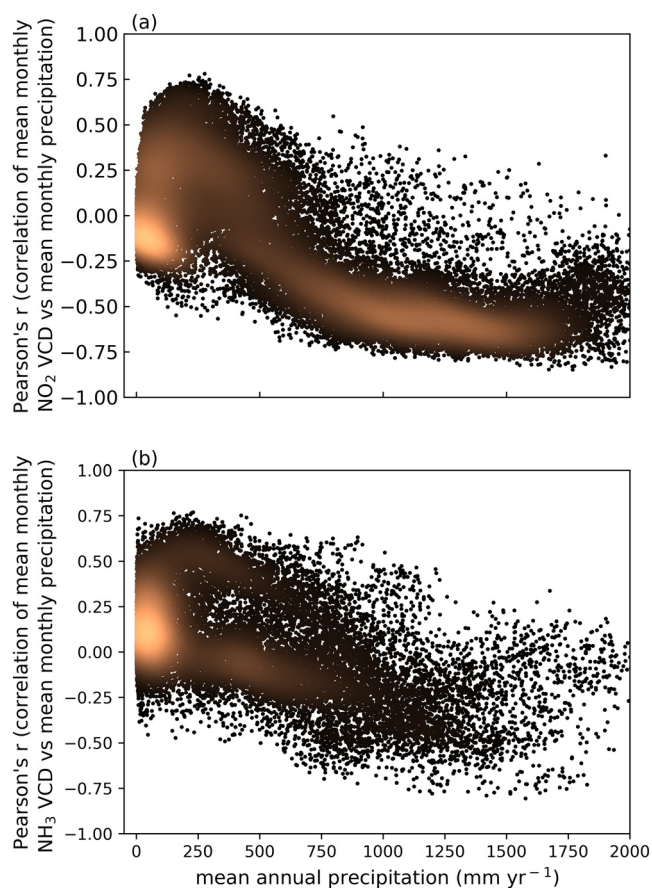
Figure 3. Mean annual precipitation (MAP, mm yr -1 ) determines the direction and strength of the correlation between mean monthly precipitation and (a) mean monthly tropospheric nitrogen dioxide (NO 2 ) vertical column density (VCD) (2005–2017) and (b) mean monthly atmospheric ammonia (NH 3 ) VCD (2008–2017) for 0.25° grid cells over all of continental Africa. Precipitation values are from Tropical Rainfall Measuring Mission, and NO 2 and NH 3 data are from Ozone Monitoring Instrument and Infrared Atmospheric Sounding Interferometer, respectively. Lighter shades of copper represent a higher density of grid cells.
