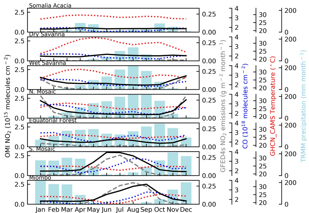
Figure 4. Seasonal variability in nitrogen dioxide ( \text{NO}_2 ) vertical column densities (VCDs) and related variables or drivers for seven major ecoregions in sub-Saharan Africa, 2005–2017. Total monthly precipitation (blue bars, \text{mm month}^{-1} ) and mean monthly surface temperature (dotted red line, ^{\circ}\text{C} ), tropospheric \text{NO}_2 VCDs (solid black line, 10^{15} molecules \text{cm}^{-2} ), atmospheric carbon monoxide (CO) VCDs (dotted blue line, 10^{18} molecules \text{cm}^{-2} ), and biomass burning emissions of \text{NO}_2 (dashed gray line, \text{g m}^{-2} \text{month}^{-1} ) are presented. GHCN_CAMS, Global Historical Climatology Network version 2 and the Climate Anomaly Monitoring System; OMI, Ozone Monitoring Instrument; TRMM, Tropical Rainfall Measuring Mission.
