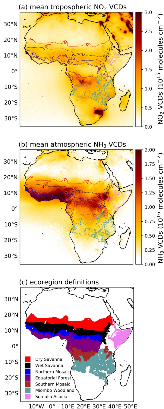
Figure 1. Mean annual nitrogen dioxide ( \text{NO}_2 ) and ammonia ( \text{NH}_3 ) vertical column densities (VCDs) and ecoregion definitions. (a) Long-term mean tropospheric \text{NO}_2 VCDs as observed by Ozone Monitoring Instrument (2005–2017). (b) Long-term mean atmospheric \text{NH}_3 VCDs as observed by Infrared Atmospheric Sounding Interferometer (2008–2017). (c) Boundaries of seven major African ecoregions evaluated in this study. Long-term mean VCD values are calculated from the monthly means.
