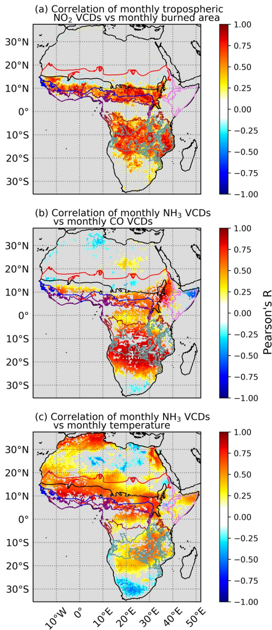
Figure 6. Map of correlation coefficients for the relationship between (a) mean monthly tropospheric nitrogen dioxide (NO 2 ) vertical column densities (VCDs) and burned area (2005–2017), (b) mean monthly atmospheric ammonia (NH 3 ) and carbon monoxide (CO) VCDs (2008–2017), and (c) mean monthly atmospheric NH 3 VCDs and land surface temperature (2008–2017) overlaid with ecoregion boundaries. Values are included only over land where the relationship is significant at p < 0.05 . Additional analyses for NH 3 VCDs and burned area, NO 2 and CO VCDs, and NO 2 and NH 3 VCDs and AOD are included as Figures S1b, S4, and S6–S8.
