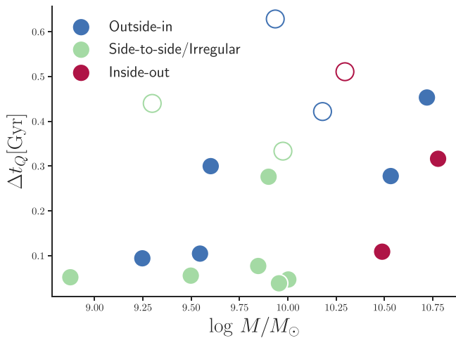
Figure 8. Log stellar mass ( \log M/M_{\odot} ) vs. the variation of t_Q within each galaxy ( \Delta t_Q ). Colors indicate the quenching direction measured from the \mu_{1.5} and t_Q maps. Galaxies without a clear enhancement of SFR prior to quenching are shown as open circles.
