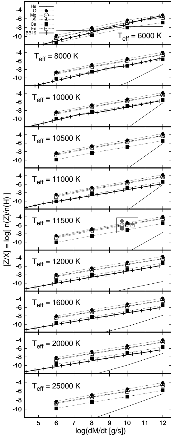
Fig. 11. Same as Fig. 10 but for models with M_H = 10^{-6} M_\odot . When possible, ^{40}\text{Ca} abundances obtained by Bauer & Bildsten (2019) have been added to the corresponding panel (labeled as BB19). For T_{\text{eff}} = 11\,500\text{ K} , gray symbols (inside a box) represent the abundances obtained by Bauer & Bildsten (2018) for ^{16}\text{O} , ^{24}\text{Mg} , ^{28}\text{Si} , ^{40}\text{Ca} , and ^{56}\text{Fe} using the observed photospheric abundance of pollutants in G29–38. All these isolated points correspond to an accretion rate of 10^{10}\text{ g s}^{-1} but have been shifted a bit from that particular value for the sake of clarity.
