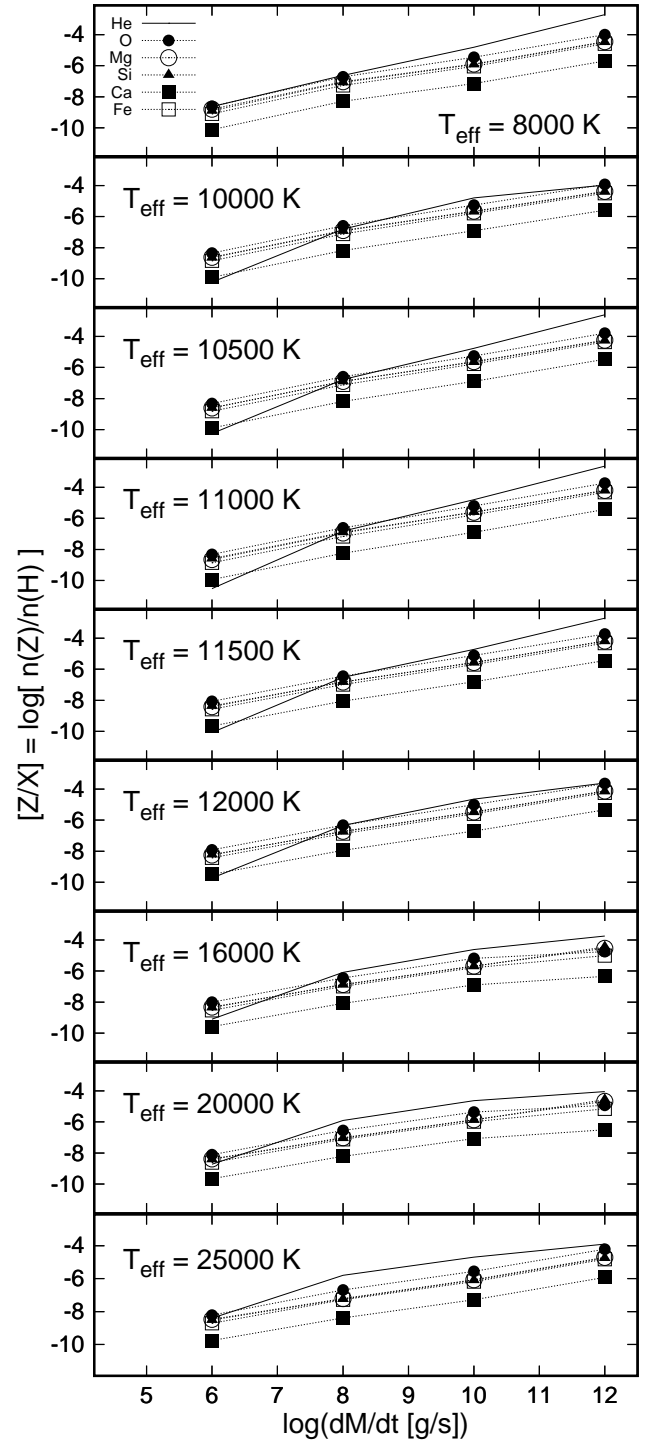
Fig. A.1. Same as Fig. 10 but for models with M_H = 10^{-8} M_\odot .
