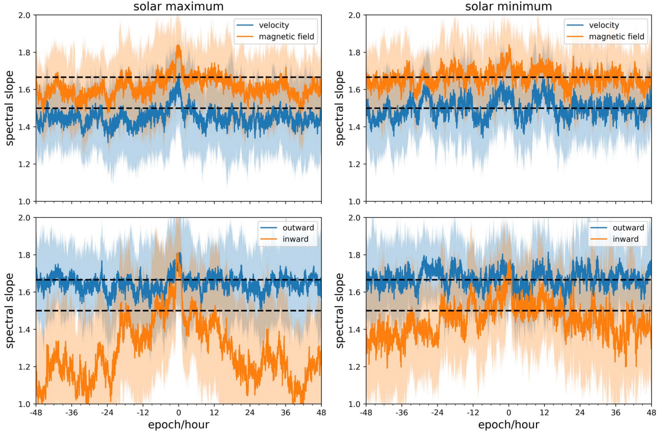
Figure 9. Superposed-epoch analysis of various spectral slopes near HCS. Top panels show slopes of velocity (blue) and magnetic field (orange), and bottom panels show slopes of outward (blue) and inward (orange) Elsässer variables. Left column is solar maximum and right column is solar minimum. In each panel, the two horizontal lines mark the values 3/2 and 5/3 for reference. The shaded bands show the standard deviations of different curves.
