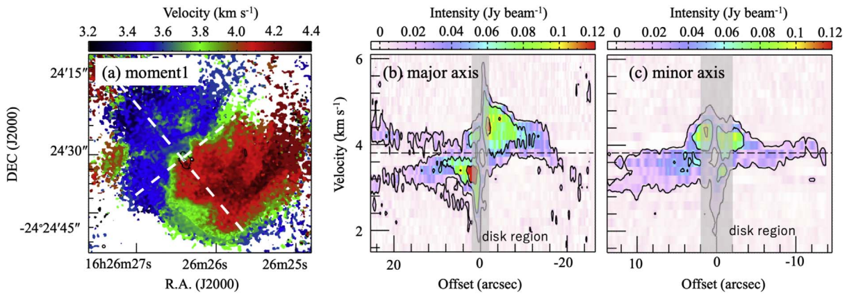
Figure 13. (a) Moment 1 map from Figure 12, and PV diagrams of the \text{H}^{13}\text{CO}^+ ( J = 3-2 ) emission along (b) the major axis and (c) the minor axis. The shadows shown in panels (b) and (c) indicate the circumbinary disk region. Contours are 0.01, 0.05, and 0.1 \text{Jy beam}^{-1} . Horizontal dashed lines show the systemic velocity ( V_{\text{sys}} = 3.8 \text{ km s}^{-1} ).
