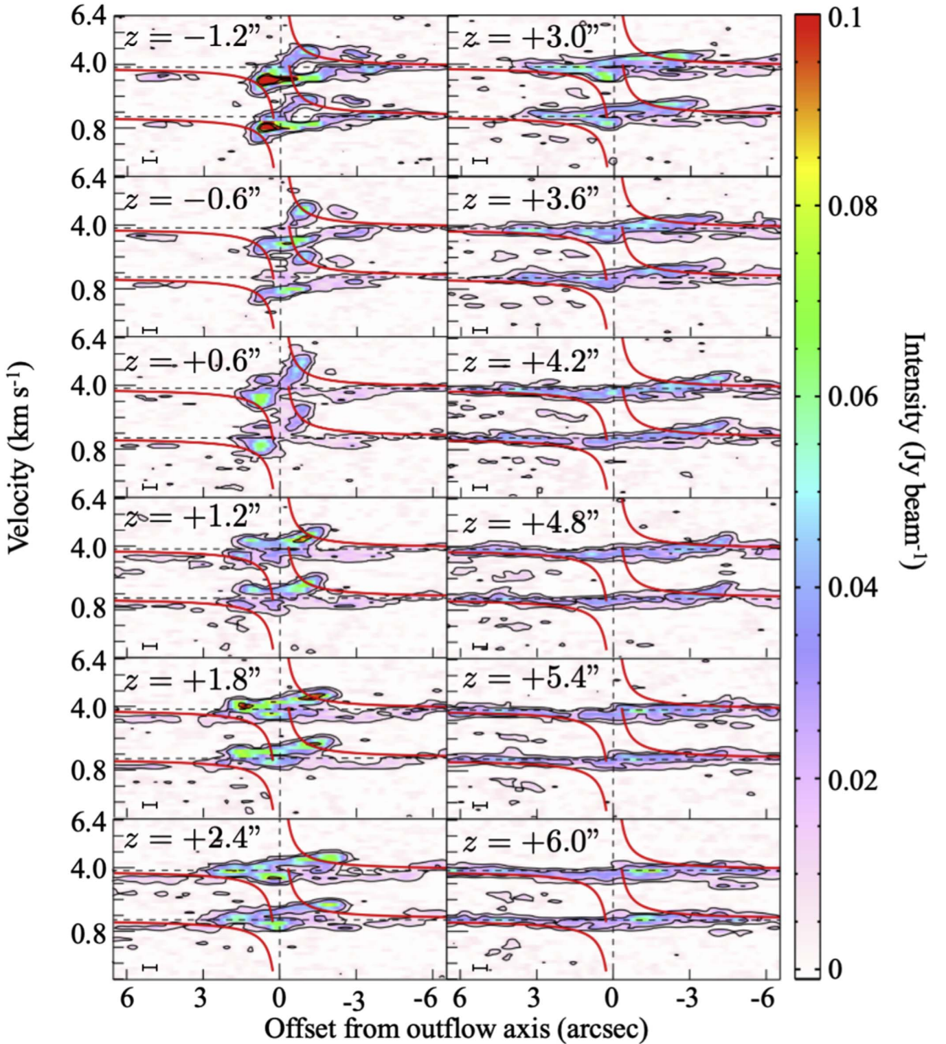
Figure 17. PV diagrams of the CCH ( N = 3 - 2 , J = 5/2 - 3/2 ) emission along the lines perpendicular to the outflow axis (shown in Figure 16). The distances of these lines to the central source are labeled in the upper left corner of each panel ( z > 0 for the southeast lobe and z < 0 for the northwest lobe). The contours are 6, 20, 80, and 100 mJy beam ^{-1} . The rest frequency of the F = 4-3 hyperfine line is used, so that the F = 3-2 hyperfine line appears at a blueshifted velocity. The red curves correspond to a constant angular momentum of 100 au km s ^{-1} (see Section 4.4.2). The black bar in the lower right corner of each panel indicates the beam size.
