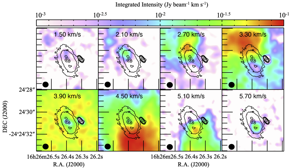
Figure 8. The same channel maps of the \text{H}^{13}\text{CO}^+ ( J = 3-2 ) emission as Figure 7, but zoomed-in views around the protostars. The black contours indicate the 0.87 mm dust continuum emission (Harris et al. 2018) to indicate the disks and stellar positions. The contour levels are the same as in Figure 1. The beam size is shown in the lower left corners.
