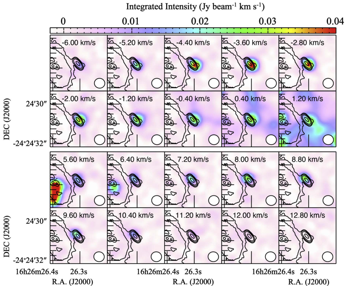
Figure 19. Channel maps of the CS emission from the high-velocity components, overlaid with the 0.87 mm dust continuum emission (Harris et al. 2018) in black contours. The channel width and step are 0.8 \text{ km s}^{-1} , and the channel centroid velocities are labeled at the upper center of each panel. The beam size is shown in the lower right corners.
