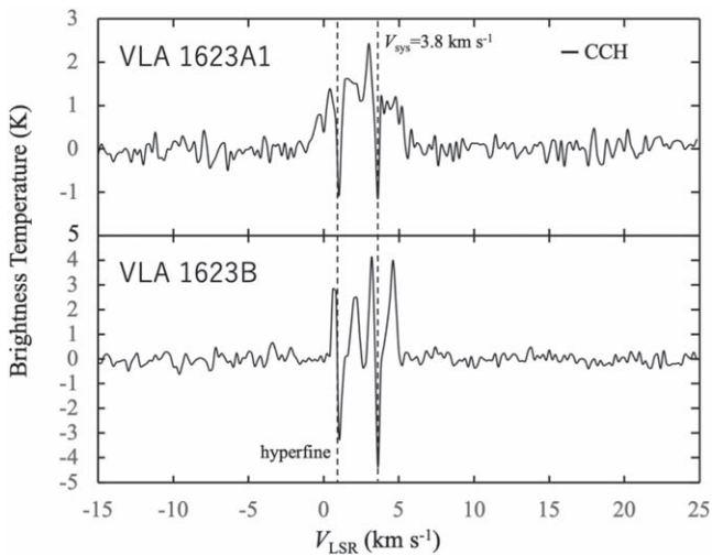
Figure 4. CCH ( N = 3-2 , J = 7/2-5/2 , F = 4-3 ) and ( N = 3-2 , J = 7/2-5/2 , F = 3-2 ) spectra toward the protostellar positions of VLA 1623A1 and VLA 1623B are shown. Vertical dashed lines stand for the source systemic velocity ( 3.8 \text{ km s}^{-1} ) relative to the F = 4-3 and F = 3-2 hyperfine components. V_{\text{LSR}} is calculated by using the F = 4-3 hyperfine component.
