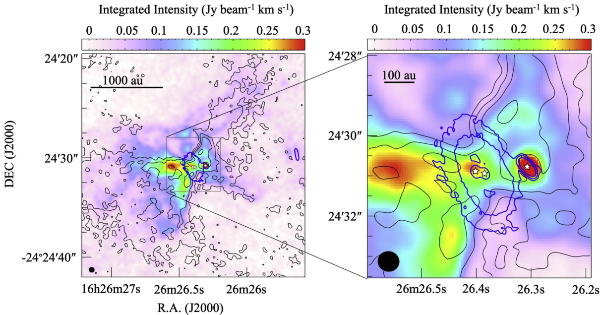
Figure 6. Integrated intensity maps of the CS emission in color scale and the CCH emission in black contours toward the VLA 1623 region. The velocity range for integration is -6 to +10 \text{km s}^{-1} . The contours of the CCH emission are 0.02, 0.05, 0.1, and 0.2 \text{Jy beam}^{-1} \text{km s}^{-1} , where 1\sigma = 0.0025 \text{Jy beam}^{-1} \text{km s}^{-1} . The blue thick contours show the 0.87 mm dust continuum emission (Harris et al. 2018) to indicate the circumbinary disk and protostellar positions. The beam size of the CS emission is shown in the lower left corner of each panel.
