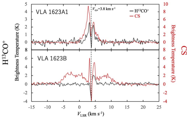
Figure 3. \text{H}^{13}\text{CO}^+ ( J = 3-2 ) and CS ( J = 5-4 ) spectra toward the protostellar positions of VLA 1623A1 and VLA 1623B are shown as the black and red lines, respectively. Vertical dashed lines stand for the source systemic velocity ( 3.8 \text{ km s}^{-1} ).
