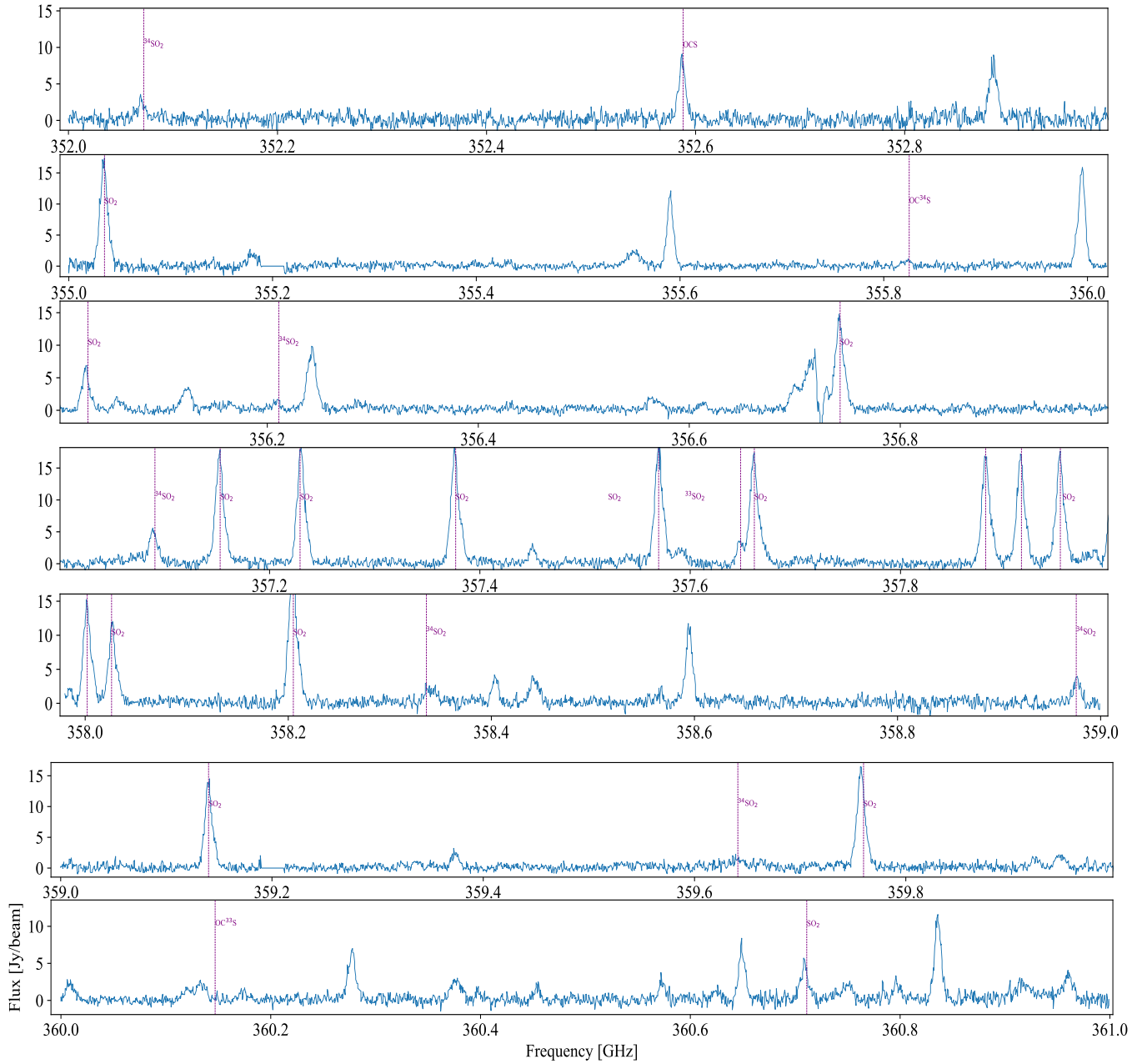
Fig. C.7. Spectrum in the range 352–361 GHz toward the source CygX-N30. Transitions of the sulphur species are identified.
