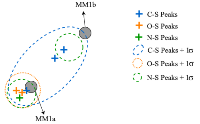
Fig. 8. Cartoon of the locations of sulphur species characterized w.r.t. chemical families (i.e., N-S, O-S and C-S) of Cyg X-N30 around the MM1 source. Concentrations of the sulphur peaks located in specific regions depending on the corresponding sulphur family. Results from the SMA-PILS Cygnus survey. Cyg X-N30 was observed at 0.8 mm.
