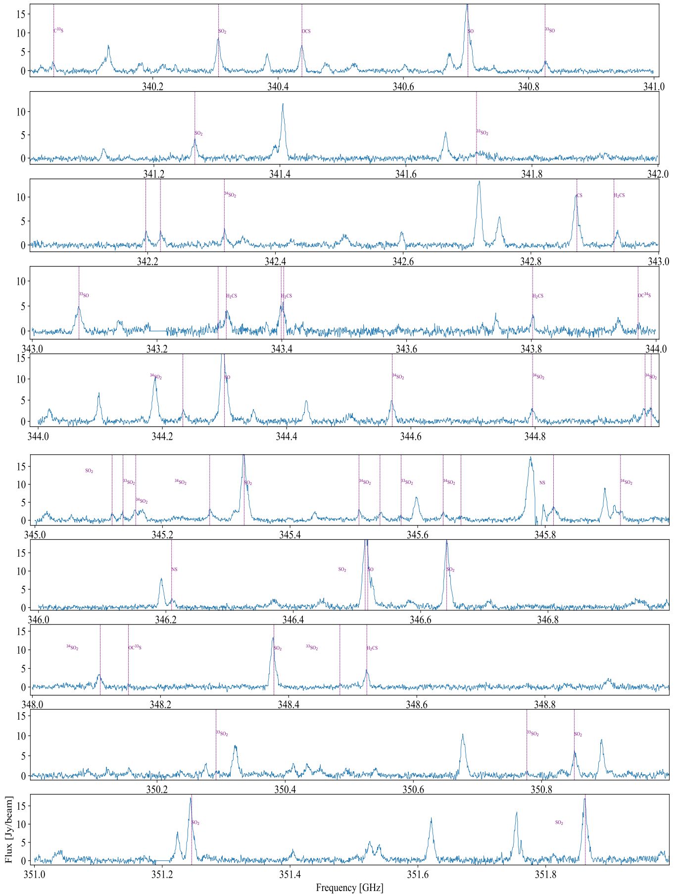
Fig. C.6. Spectrum in the range 340-352 GHz toward the source CygX-N30. Transitions of the sulphur species are identified.
