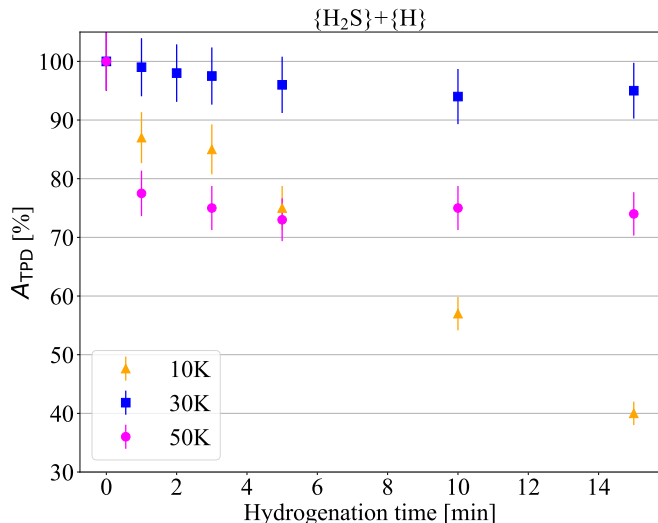
Fig. 2. Integrated area of the m/z = 34 ( \text{H}_2\text{S} ) curve as a percentage of the initial amount of \text{H}_2\text{S} injected in the experiment at each temperature. The area is calculated from the QMS while performing a TPD, resulting from hydrogenation of 1 ML of \text{H}_2\text{S} during varying time, and at varying deposition temperature of \text{H}_2\text{S} (10, 30, and 50 K).
