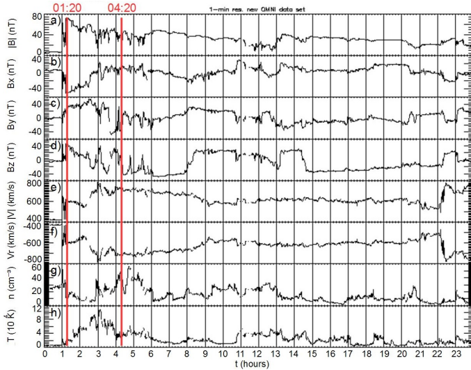
Fig. D.2. OMNIWeb data during the 31/03/2001 ICME. (a) |B| (nT), (b) B_x (nT), (c) B_y (nT), (d) B_z (nT), (e) |v| (km/s), (f) v_r (km/s), (g) n ( \text{cm}^{-3} ), and (h) T ( 10^4 K). The solid red line indicates the time frame we selected as the simulation input.
