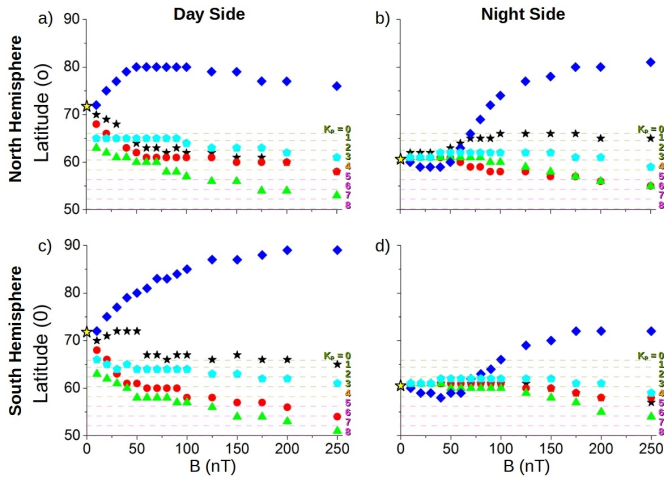
Fig. 14. OCB latitude with respect to the IMF orientation and |B_{IMF}| calculated in the North Hemisphere (a) DS ( 0^\circ longitude) and (b) NS ( 180^\circ longitude), South Hemisphere (c) DS and (d) NS. Fixed P_d = 1.2 nPa and T_{sw} = 1.8 \times 10^5 K. The dashed horizontal lines indicate the K_p index. The yellow star indicates the OCB latitude if |B_{IMF}| = 0 . IMF direction: Sun–Earth (black star), Earth–Sun (red circle), northward (blue diamond), southward (green triangle), and ecliptic ctr-clockwise (cyan pentagon).
