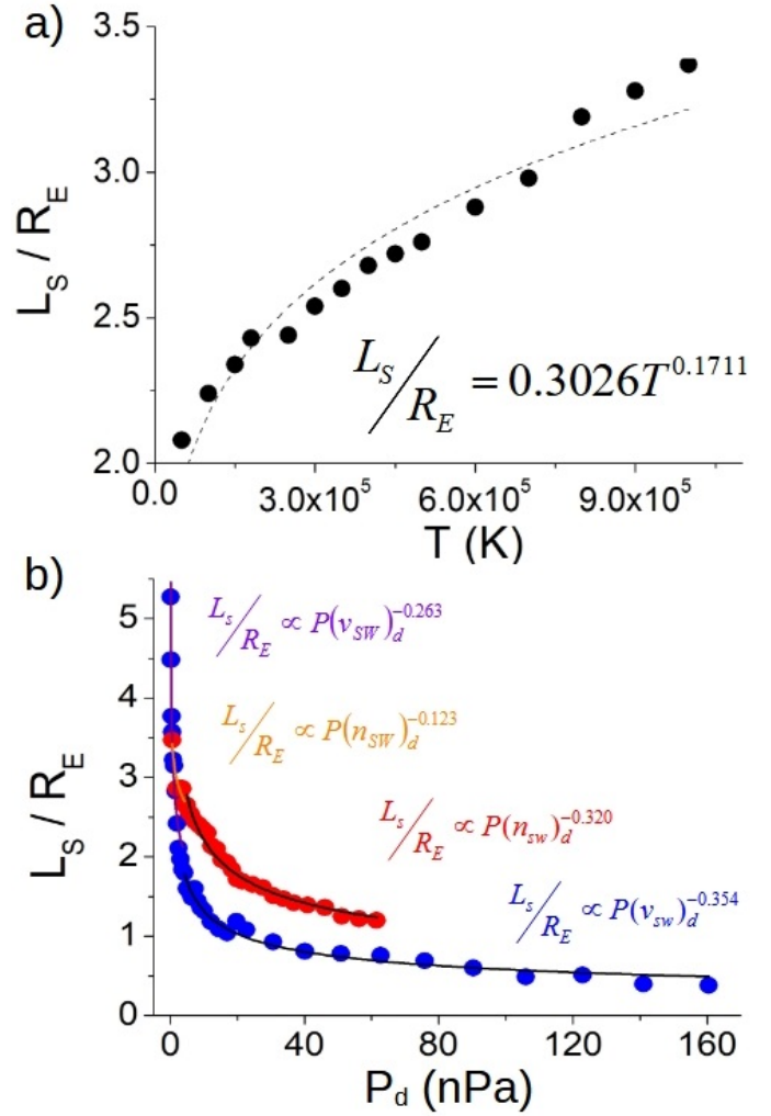
Fig. 9. BS width for (a) different SW temperatures (fixed P_d = 1.2 nPa) and (b) different P_d values (fixed T_{sw} = 1.8 \times 10^5 K) when the SW density increases (fixed the SW velocity to 350 km s -1 , red dots) or the SW velocities increases (fixed the SW density to 12 cm -3 , blue dots). Sun–Earth IMF orientation with |B| = 10 nT. The dashed lines indicate the data fit to the expression L_{bs}/R_E = AT_{sw}^\alpha . The solid black lines indicate the regression L_{bs}/R_E = AP(n_{sw})_d^\alpha in the simulations with the SW velocity fixed and P_d > 4 nPa and L_{bs}/R_E = AP(v_{sw})_d^\alpha in the simulations with the SW density fixed and P_d < 4 nPa. The solid violet (orange) line indicates the regression L_{bs}/R_E = AP(n_{sw})_d^\alpha ( L_{bs}/R_E = AP(v_{sw})_d^\alpha ) when P_d < 4 nPa.
