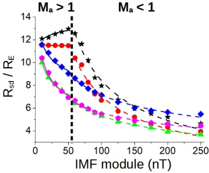
Fig. 6. Magnetopause standoff distance with respect to |B|_{\text{IMF}} when the IMF is oriented in the Sun–Earth direction (black star), Earth–Sun (red circle), northward (blue diamond), southward (green triangle), and ecliptic ctr-clockwise direction (pink hexagon). The solid (dashed) lines indicate for each IMF orientation the data fit to the expression R_{\text{sd}}/R_E = A|B|_{\text{IMF}}^\alpha of the simulations with M_a > 1 ( M_a < 1 ).
