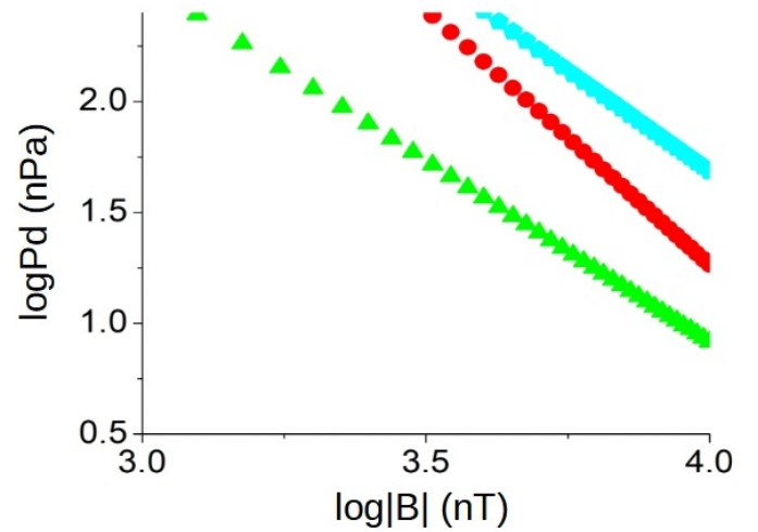
Fig. 18. Critical |B|_{\text{IMF}} required for the direct precipitation of the SW toward the Earth surface with respect to P_d and the IMF orientation. Fixed T_{\text{sw}} = 1.8 \times 10^5 K. IMF direction: Earth–Sun (red circle), southward (green triangle), and ecliptic ctr-clockwise (cyan pentagon).
