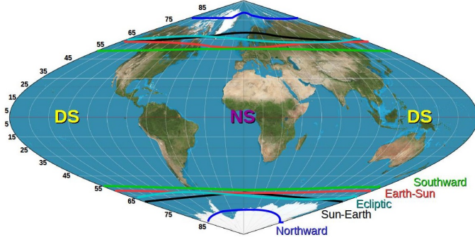
Fig. 15. Schematic view of the OCB line for Sun–Earth (black line), Earth–Sun (red line), northward (blue line), southward (green line), and ecliptic ctr-clockwise (cyan lines) with |B_{\text{IMF}}| = 250 nT. The parameters P_d = 1.2 nPa and T_{\text{sw}} = 1.8 \times 10^5 K are fixed. The location of the DS and NS with respect to the continents is irrelevant.
