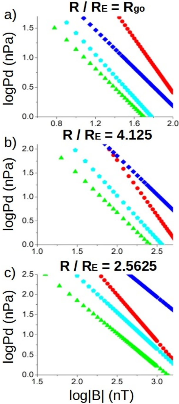
Fig. 19. Critical P_d to reduce the magnetopause standoff distance below (a) the geostationary orbit (b) medium orbit at R_{mo} = R/R_E = 4.125 and (c) medium orbit at 2.5625 for different IMF intensities and orientations. Fixed T = 1.8 \times 10^5 K. IMF direction: Earth–Sun (red circle), northward (blue diamond), southward (green triangle), and ecliptic counter-clockwise (cyan pentagon).
