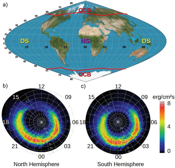
Fig. 22. (a) OCB line calculated from the 27/05/2017 ICME simulation. Energy flux calculated by Ovation prime simulations at the (b) North Hemisphere and (c) South Hemisphere. Ovation prime data are provided by the iSWA (iSW 2020).
