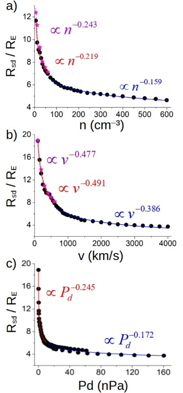
Fig. 8. Magnetopause standoff distance with respect to (a) the SW density (fixed v = 350 km s ^{-1} ), (b) SW velocities (fixed 12 cm ^{-3} ), and (c) dynamic pressure. Sun–Earth IMF orientation with |B| = 10 nT. The pink stars indicate the magnetopause standoff distance if |B| = 0 nT. The dashed lines indicate the data fit to the expression R_{\text{sd}}/R_E = An^\alpha , R_{\text{sd}}/R_E = A|v|^\alpha , and R_{\text{sd}}/R_E = AP_d^\alpha . The solid red line indicates the fit line for the data set with n \leq 60 cm ^{-3} and |v| \leq 600 km s ^{-1} . The solid blue line indicates the fit line for the data set with n > 60 cm ^{-3} and |v| > 600 km s ^{-1} . The solid pink line indicates the fit line for the data set with n \leq 60 cm ^{-3} and |v| \leq 600 km s ^{-1} and no IMF.
