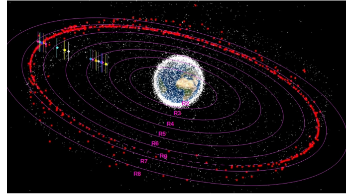
Fig. 23. Schematic view of the satellites at geosynchronous, high, medium, and low orbits around the Earth between 2000–2020. The orbits highlighted by red dots are geosynchronous satellites. The solid pink lines indicate orbits at R/R_E = i with i an integer between 2 to 8 ( R_i ). The dashed pink line indicates the geosynchronous orbit ( R_g ). The colored symbols and horizontal lines show the standoff distance of the magnetopause and the BS nose for the different ICMEs we analyzed: light green star for 22/10/1999, light cyan star for 16/07/2000, light pink star for 31/03/2001b, light gray star for 24/11/2001, yellow diamond for 29/05/2003, cyan diamond for 24/10/2003, pink diamond for 07/11/2004, gray diamond for 21/01/2005, orange triangle for 15/05/2005, and blue triangle for 24/08/2005.
