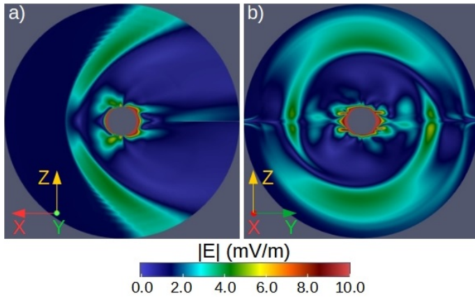
Fig. A.2. Electric field module in the simulation domain for the benchmark case in Samsonov et al. (2016) in (a) the XZ plane and (b) in the YZ plane.
