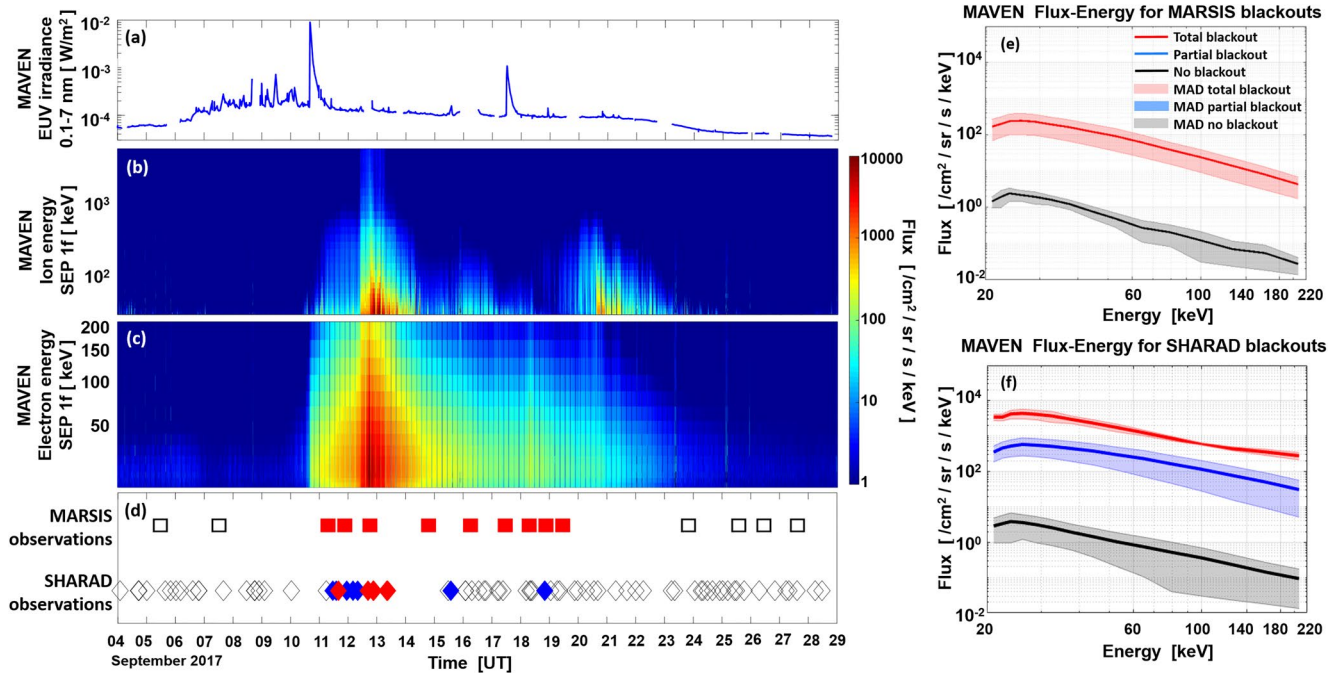
Figure 6. Case Study 1 (4 September to 29 September 2017). Panel a presents MAVEN EUVM irradiance observations. Panel b presents MAVEN SEP ion spectra. Panel c presents MAVEN Solar Energetic Particle (SEP) electron spectra. Panel d presents times of MARSIS (squares) and SHARAD (diamonds) operations. Red filled squares/diamonds represent a total blackout. Blue filled squares/diamonds represents a partial blackout. Panel e presents the median SEP electron energy flux curves for MARSIS (red curve for total blackouts, black curve for no blackouts). Panel f presents the median SEP electron energy flux curves for SHARAD (red curve for total blackouts, blue curve for partial blackouts, black curve for no blackouts). The shadow areas represent the median absolute deviation (MAD). Note that a color blind friendly version is available at https://doi.org/10.25392/leicester.data.15097008 .
