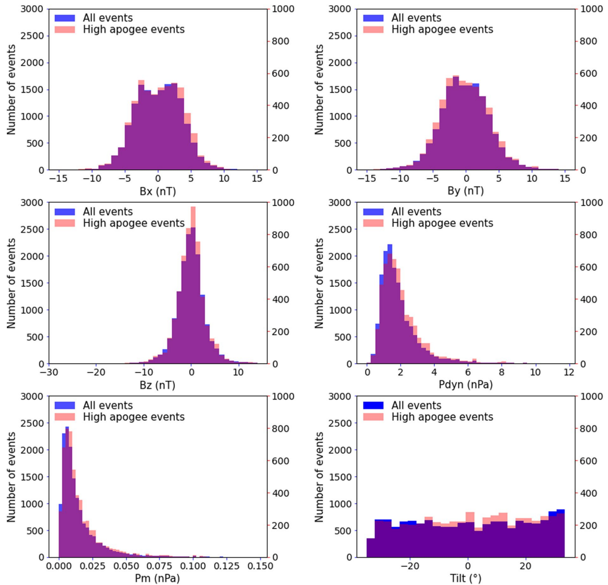
Figure 3. Histogram of the solar wind parameters of the 17,230 magnetopause crossings. Each panel is the same than in Figure 1. The red here bins show the same distribution for the events measured by high apogee spacecraft.
