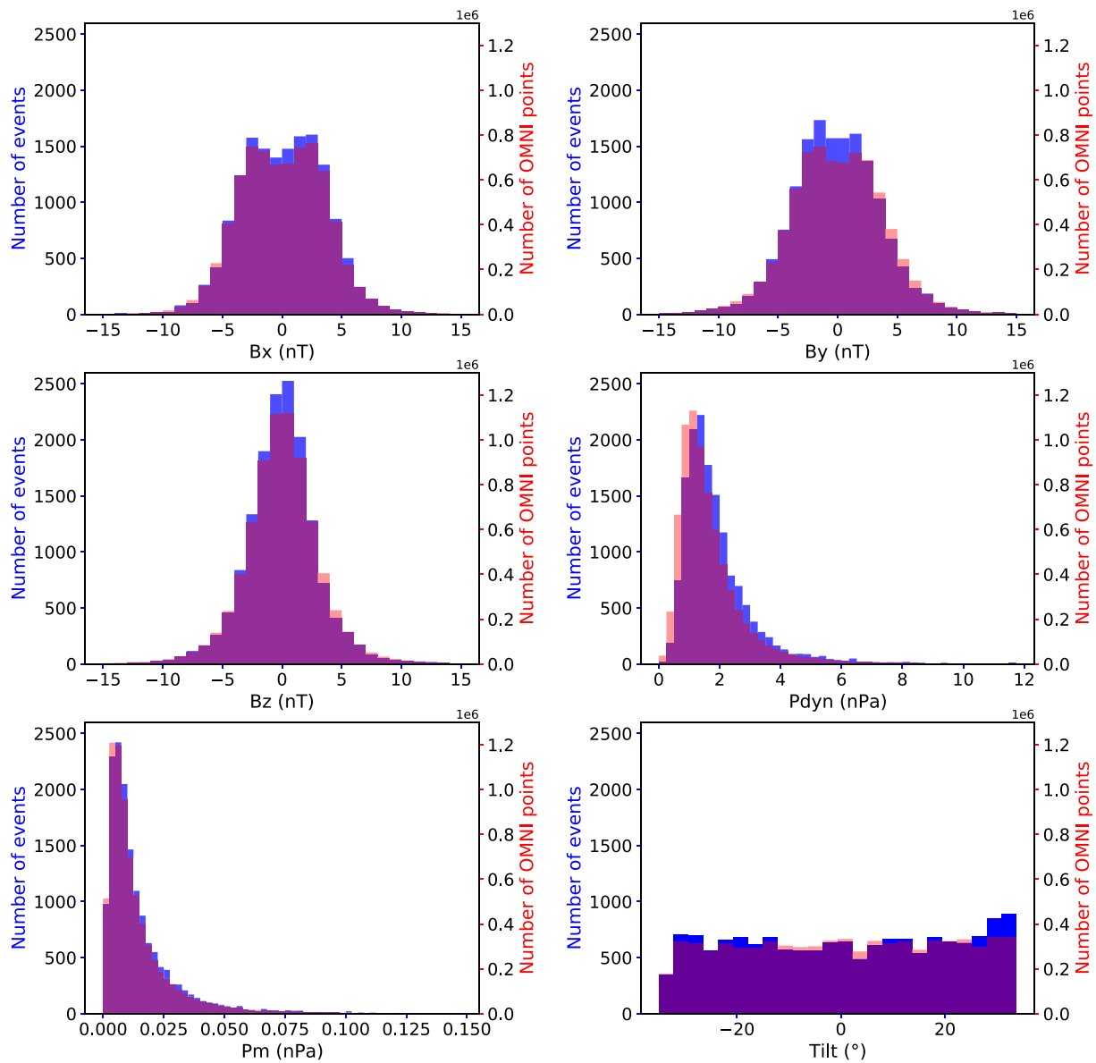
Figure 1. Statistical distribution of the solar wind parameters of the 17,230 magnetopause crossings: the three magnetic field components, B_x (top left), B_y (top right), B_z (middle left), the dynamic pressure P_{dyn} (middle right), the magnetic pressure P_m (bottom left) and the dipole tilt angle (bottom right). The red bins indicate the counterpart distribution of the physical parameters of OMNI data between 2001 and 2019.
