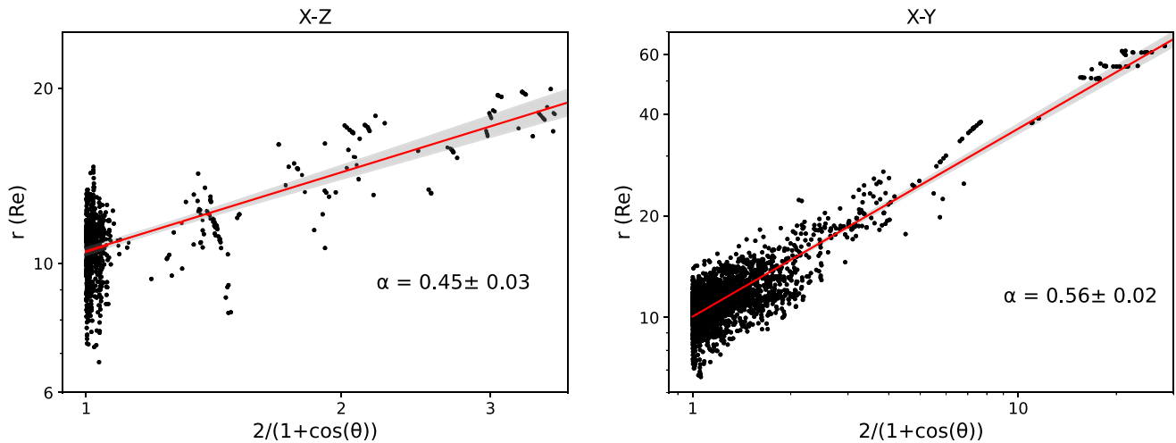
Figure 7. Evolution of the radial distance r of the crossings in the (X - Z) (left) plane and in the (X - Y) plane as a function of the inverted trigonometric function \frac{2}{1+\cos(\theta)} on a logarithmic scale. The solid red line represent the linear fit of \log r as a function of \frac{2}{1+\cos(\theta)} . The gray intervals represent the confidence intervals of such fits.
