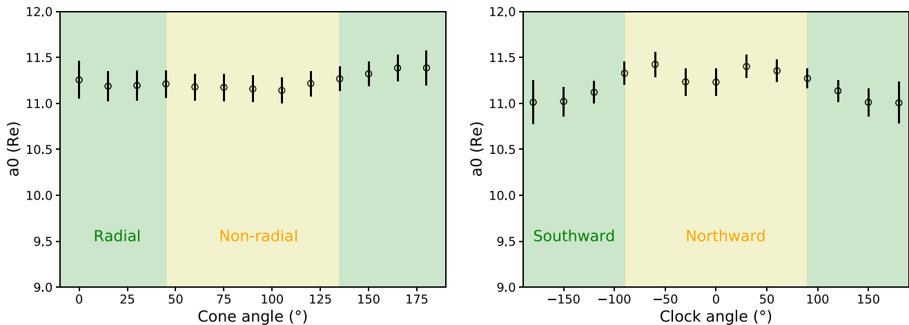
Figure 5. Evolution of the stand-off distance at 1 nPa, a_0 as a function of the interplanetary magnetic field cone ( left ) and clock ( right ) angles. The black circles represent the value we obtain from fitting a power law to r_0 for different cone (resp. clock) angle bins. The error bars represent the 1-sigma confidence interval of such fits.
