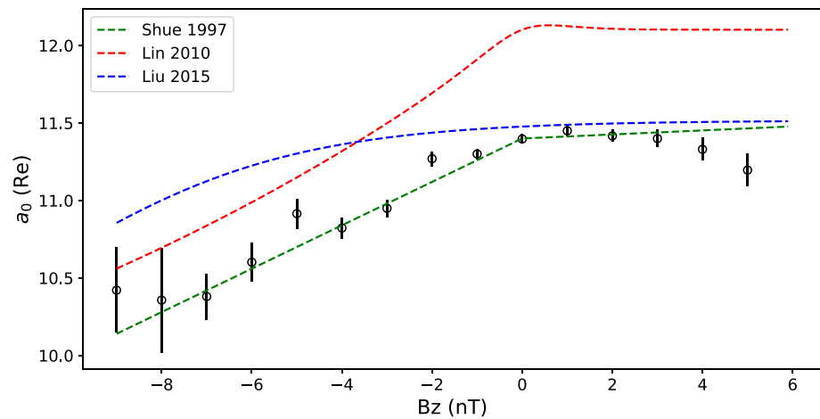
Figure 6. The same than Figure 5 but as a function of the interplanetary magnetic field B_z . The three colored dashed line represent the evolution of a_0 according three previous existing models: Shue et al. (1997) (green), Lin et al. (2010) (red) and Liu et al. (2015) (blue).
