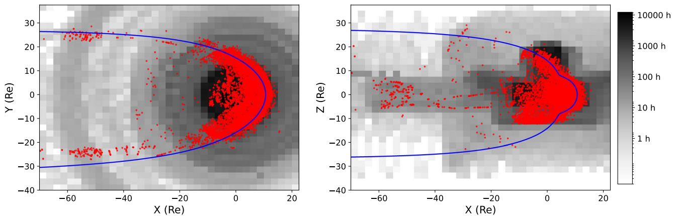
Figure 2. Projection in the (X - Y) (left) and in the (X - Z) (right) cGSM plane of the 17,230 magnetopause crossings (red dots). The gray shading represents the time spent by all of the spacecraft in a given region of the (X - Y) (resp. (X - Z) ) plane. The blue line represents Lin et al. (2010) magnetopause model with a dynamic pressure of 2 nPa and a null B_z .
