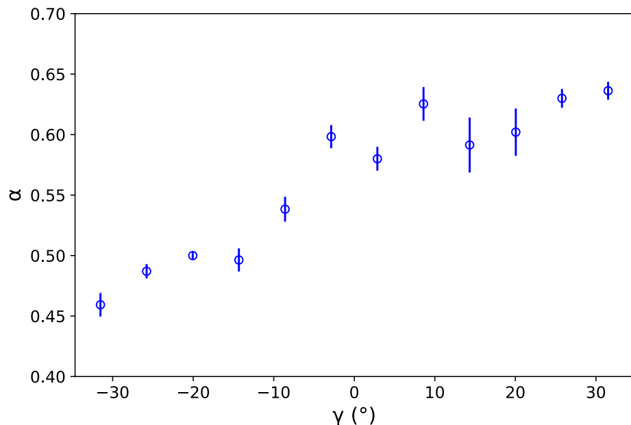
Figure 11. Evolution of the fitted flaring coefficient \alpha as a function of the dipole tilt angle \gamma for the out of cusps crossings in the (X - Z) plane. The error bars represent the 1-sigma confidence intervals of the different fits.
