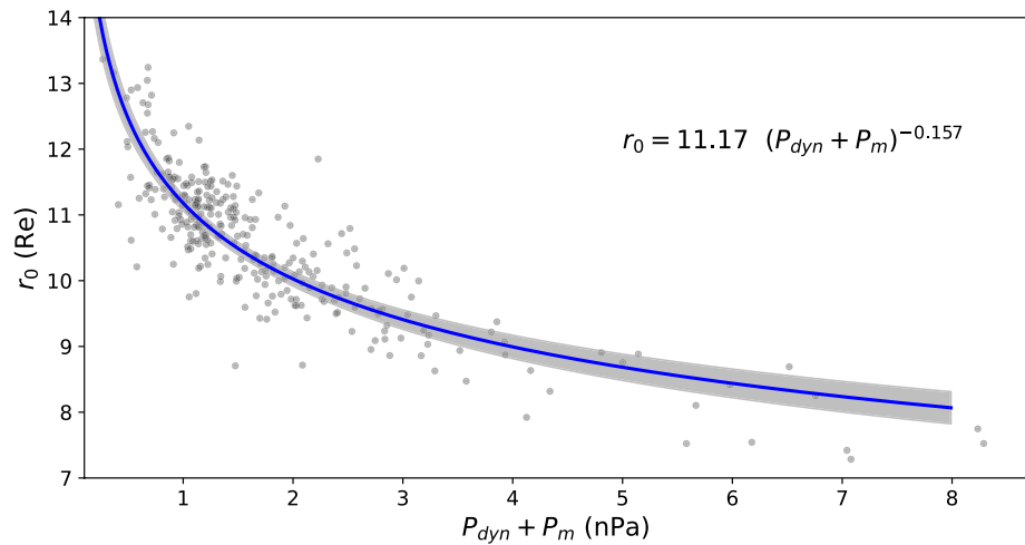
Figure 4. Variations of r_0 with the dynamic pressure. The solid blue line represent the fit of r_0 as a power-law of P_{dyn} + P_m and the gray interval is the 1-sigma confidence interval of such fit.
