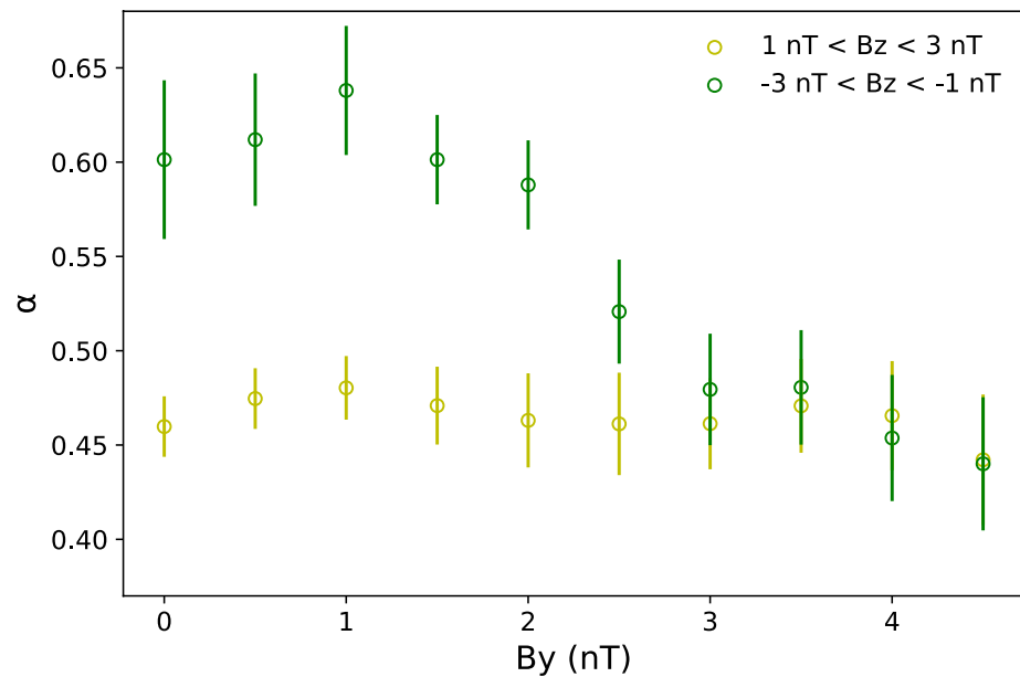
Figure 13. Evolution of the fitted flaring coefficient \alpha as a function of the interplanetary magnetic field |B_y| component for the out of cusps crossings in the (X - Z) plane for which 1 \text{ nT} < B_z < 3 \text{ nT} (yellow) and for which -3 \text{ nT} < B_z < -1 \text{ nT} (green). The error bars represent the confidence intervals of the different fits.
